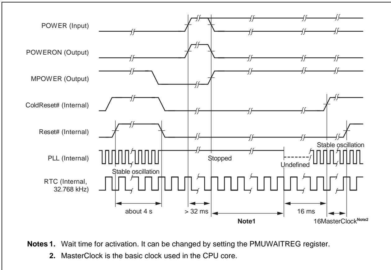
Figure 8-5. HALTimer shutdown
