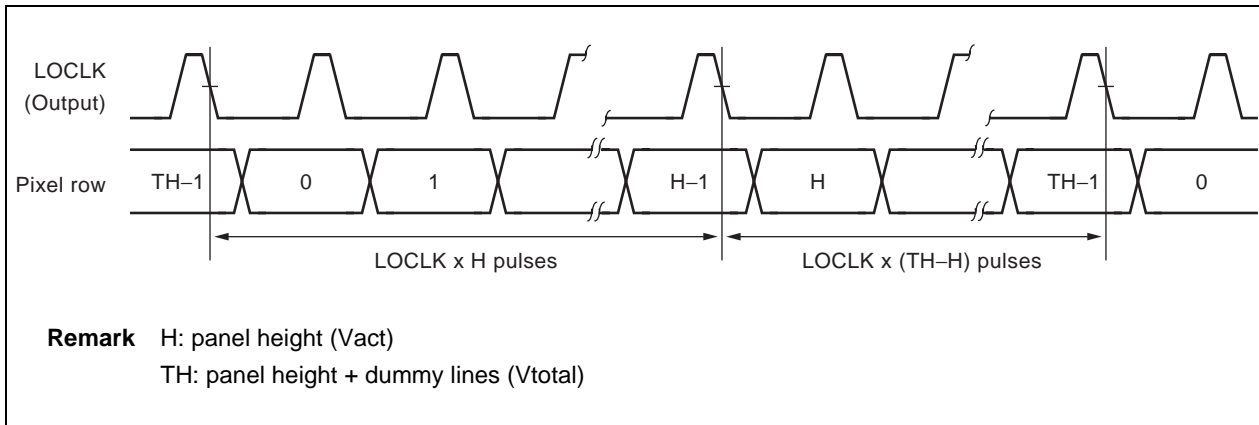
Figure 26-7. Load Clock (LOCLK)
