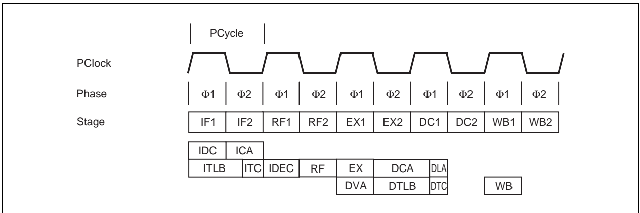
Figure 5-9. LW Instruction Pipeline Activities
