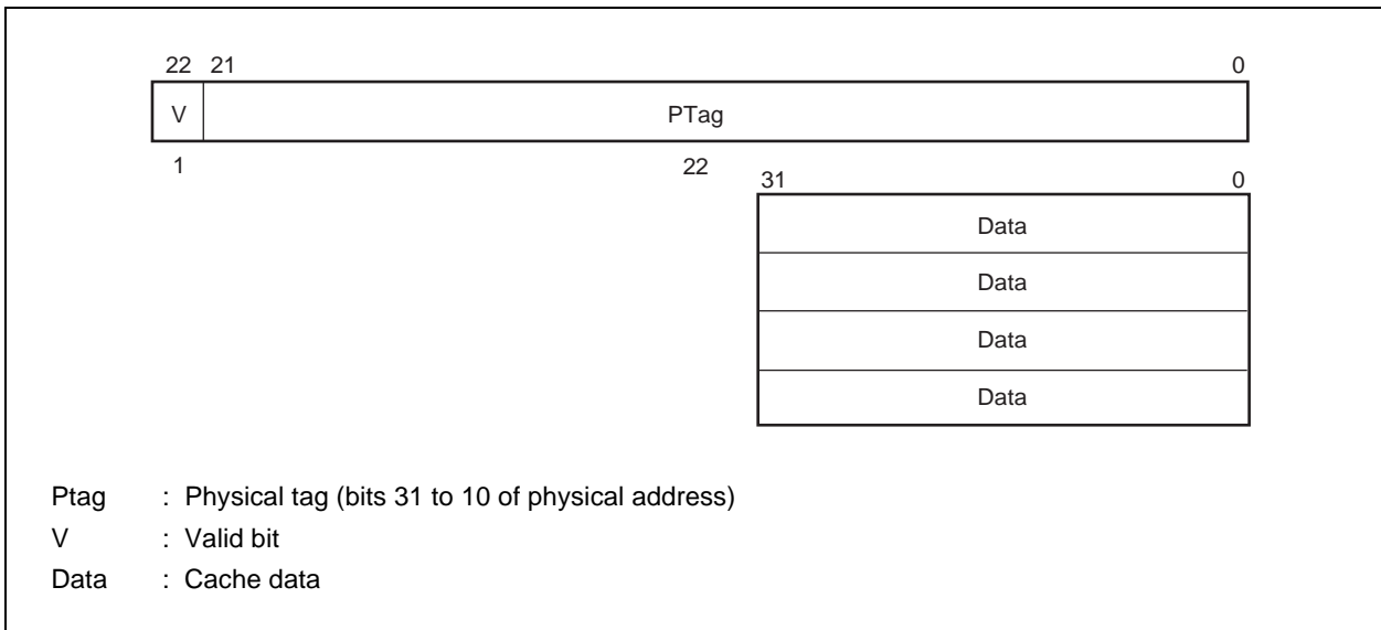
Figure 9-3. Instruction Cache Line Format
