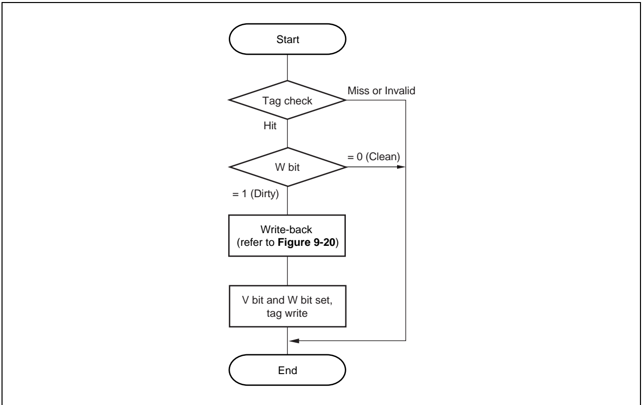
Figure 9-15. Data Check Flow on Create_Dirty Operations
