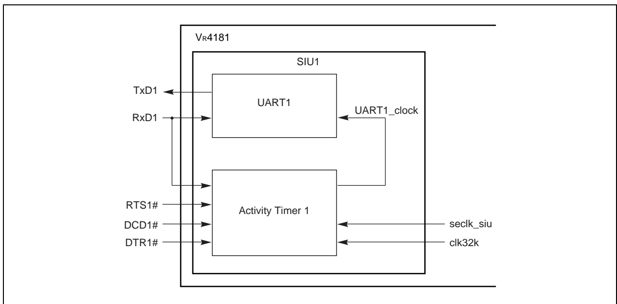
Figure 24-1. SIU1 Block Diagram
