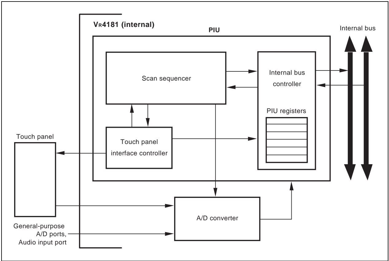
Figure 19-3. Internal Block Diagram of PIU
