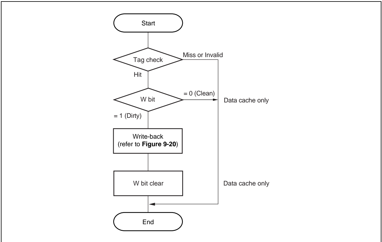
Figure 9-19. Data Check Flow on Hit_Writeback Operations
