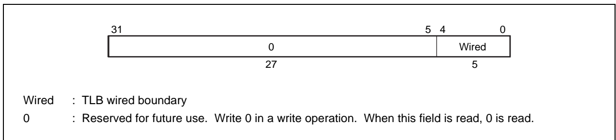
Figure 6-16. Wired Register
