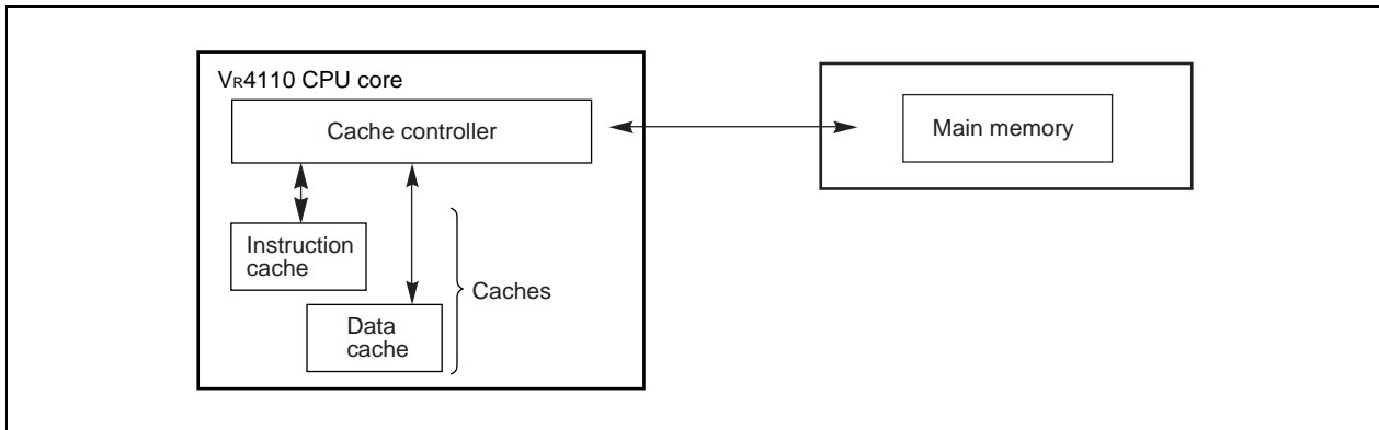
Figure 9-2. Cache Support
