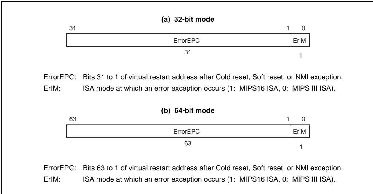
Figure 7-16. ErrorEPC Register Format (When MIPS16 ISA Is Enabled)
