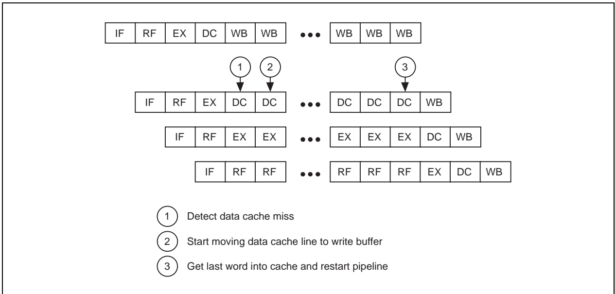
Figure 5-13. Data Cache Miss Stall
