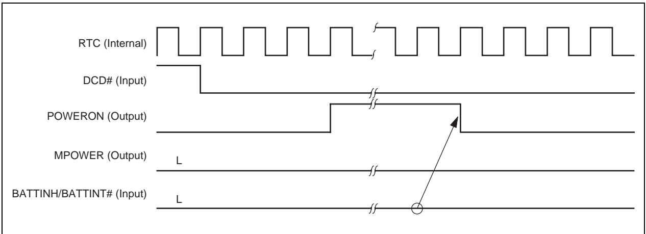
Figure 15-9. Activation via DCD Interrupt (BATTINH = L)
