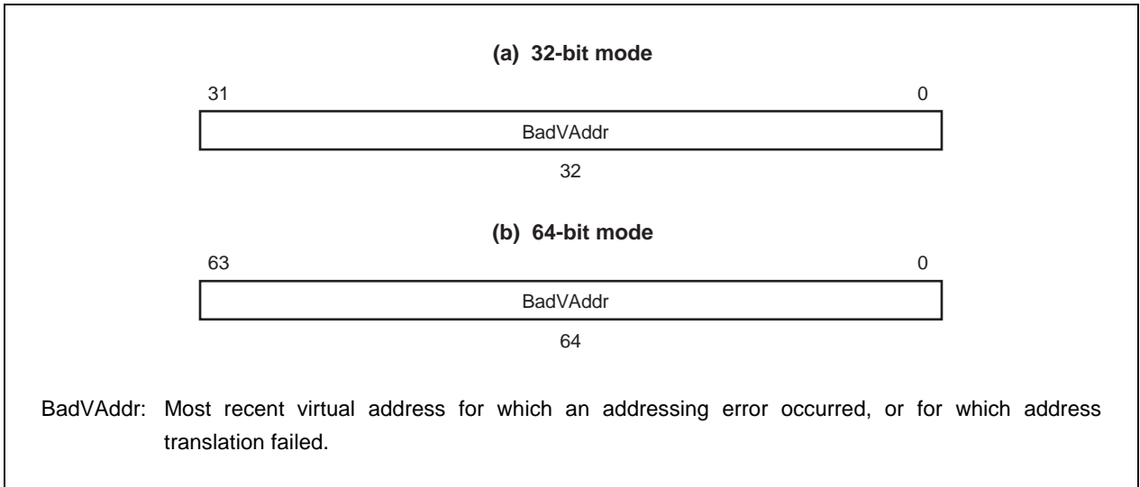
Figure 7-2. BadVAddr Register Format
