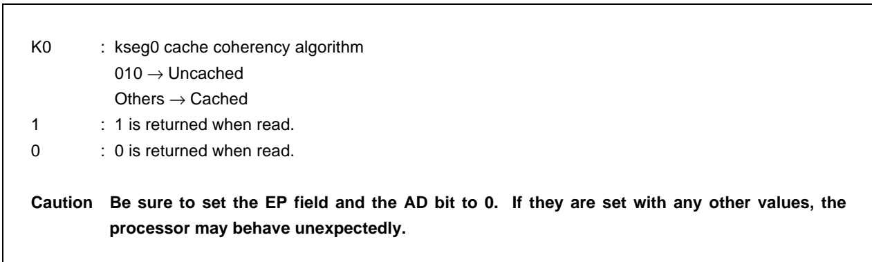
Figure 6-19. Config Register Format (2/2)
