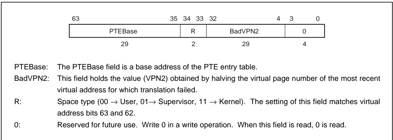
Figure 7-12. XContext Register Format
