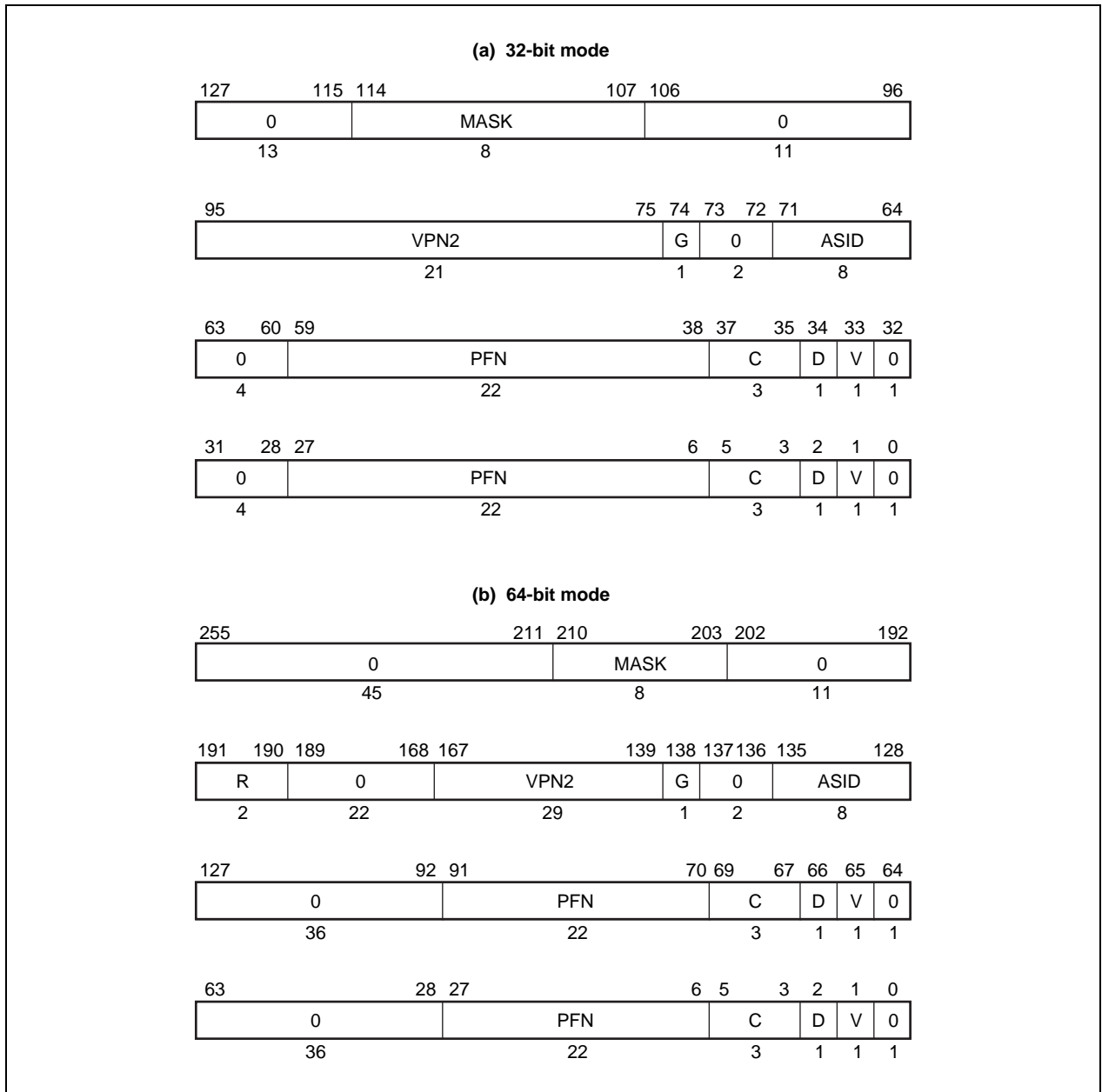
Figure 6-10. Format of a TLB Entry
