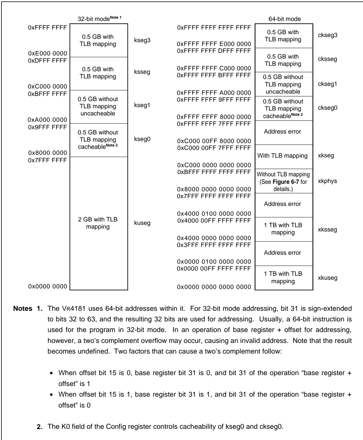
Figure 6-6. Kernel Mode Address Space
