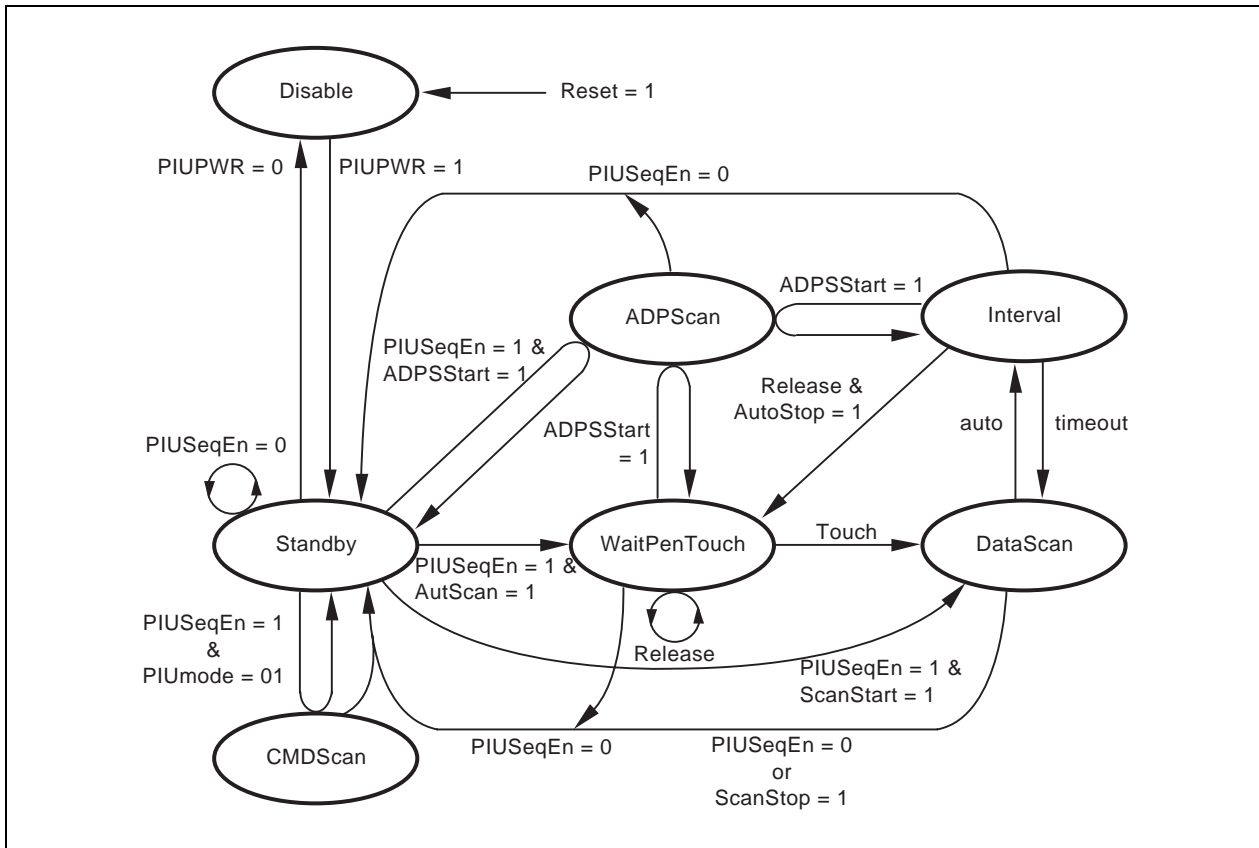
Figure 19-4. Scan Sequencer State Transition Diagram
