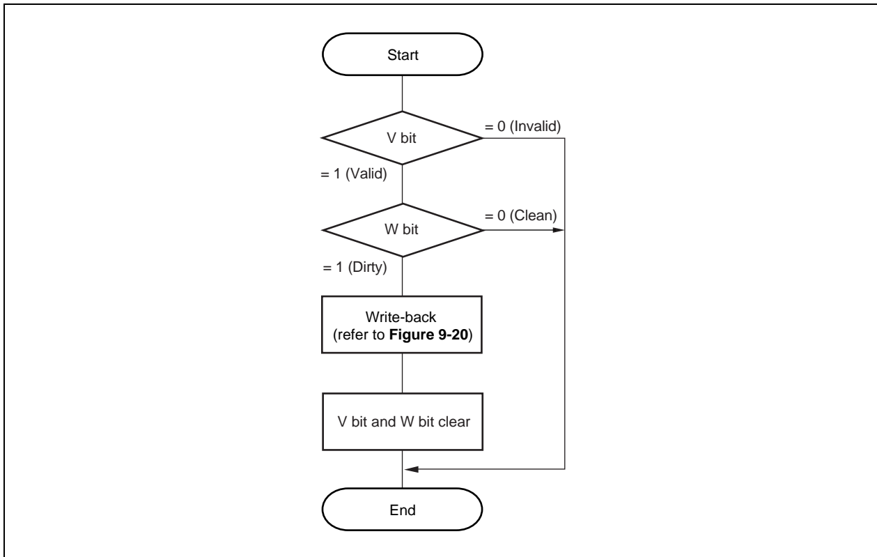
Figure 9-13. Data Check Flow on Index_Load_Tag Operations
