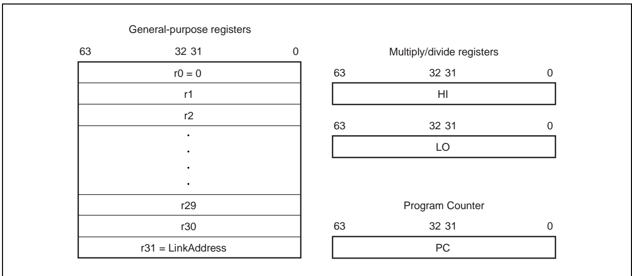
Figure 1-3. CPU Registers
