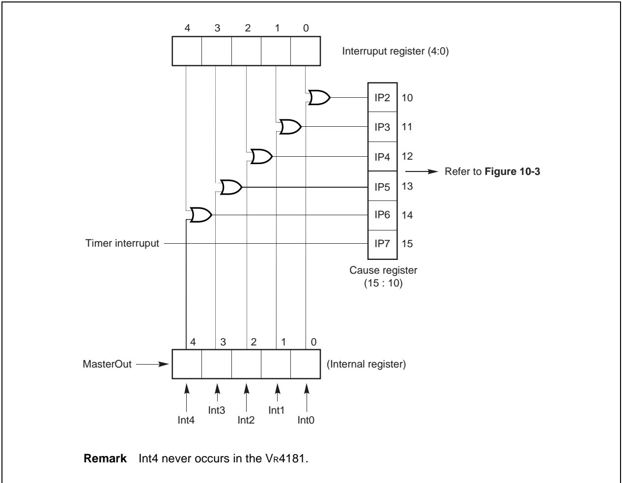
Figure 10-2. Hardware Interrupt Signals
