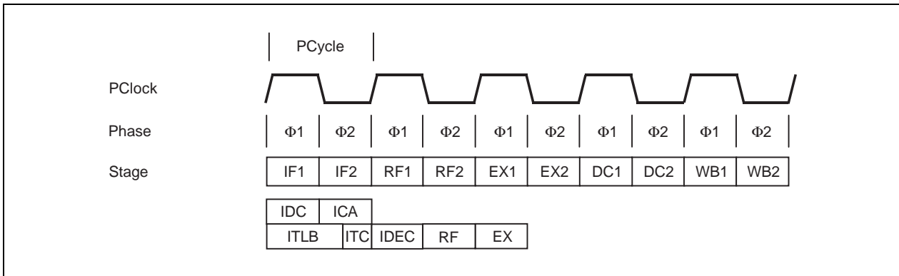
Figure 5-8. TLT Instruction Pipeline Activities
