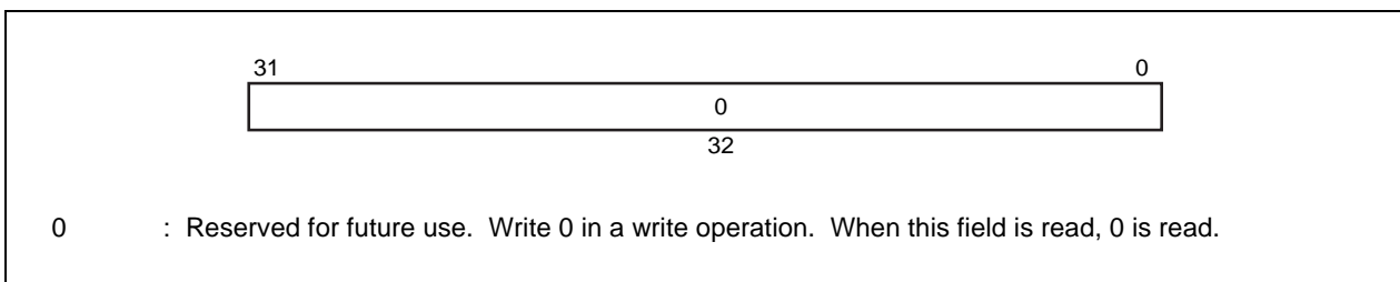
Figure 6-22. TagHi Register
