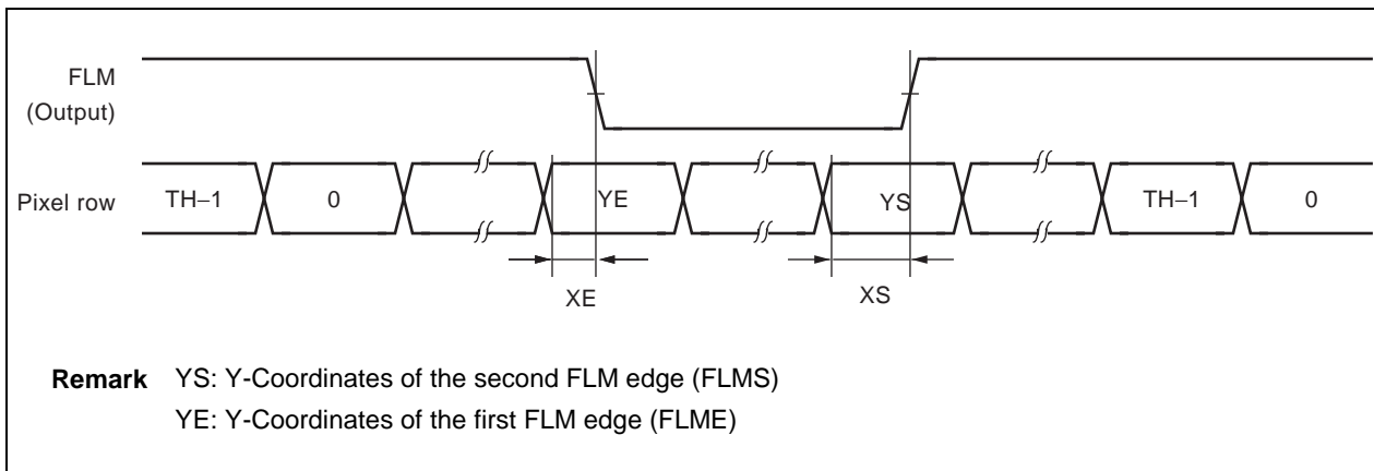
Figure 26-8. Frame Clock (FLM)
