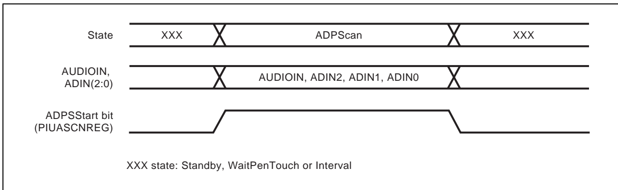
Figure 19-7. A/D Port Scan Timing
