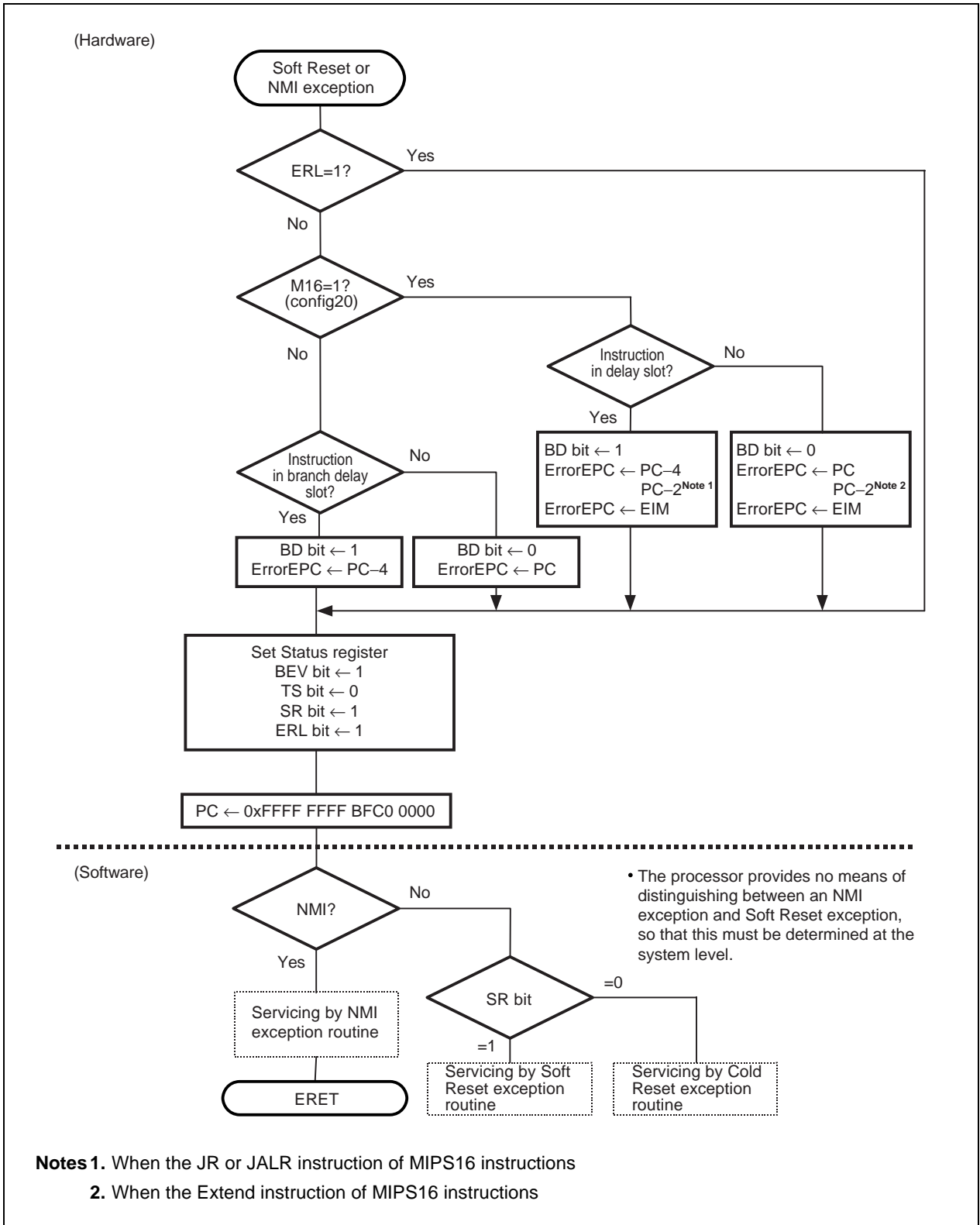
Figure 7-20. Soft Reset and NMI Exception Handling
