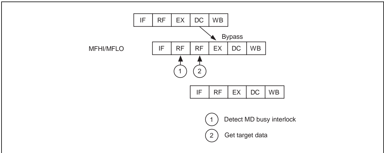
Figure 5-16. MD Busy Interlock
