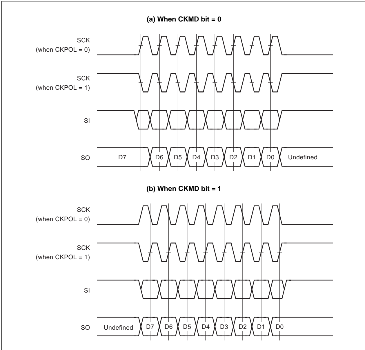
Figure 13-1. SCK and SI/SO Relationship
