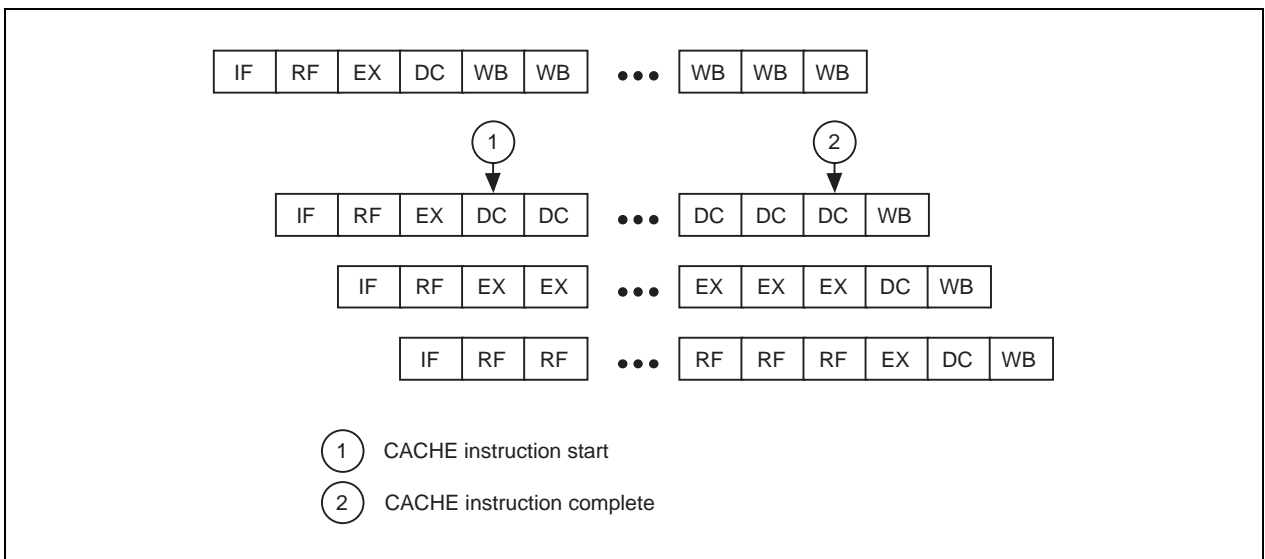
Figure 5-14. CACHE Instruction Stall
