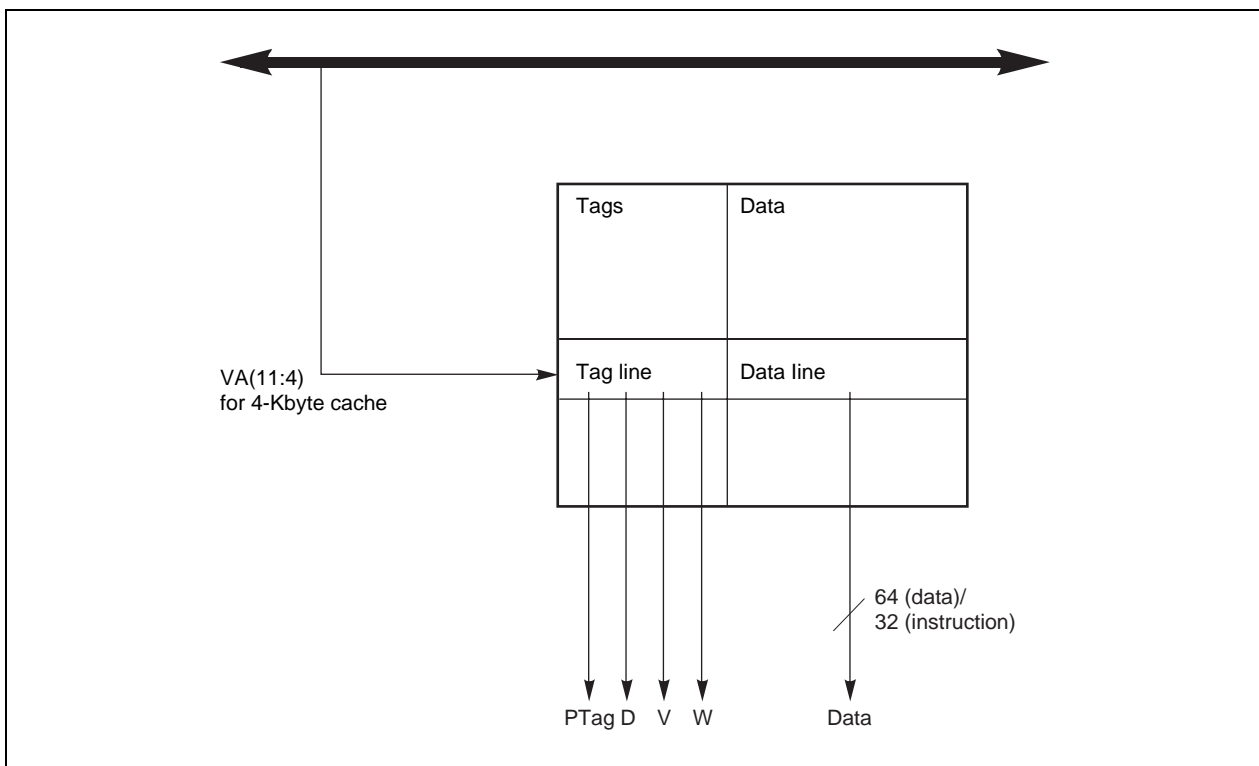
Figure 9-5. Cache Data and Tag Organization
