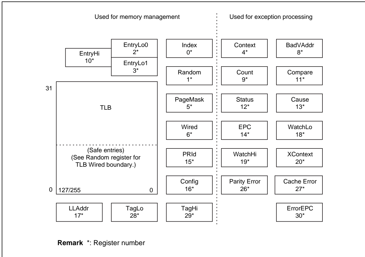
Figure 6-9. CP0 Registers and the TLB
