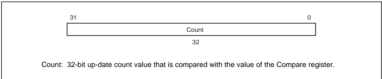
Figure 7-3. Count Register Format
