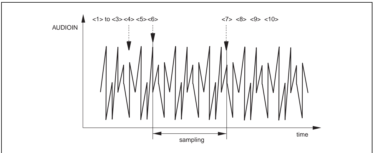
Figure 20-2. AUDIOIN Pin and Microphone Operation
