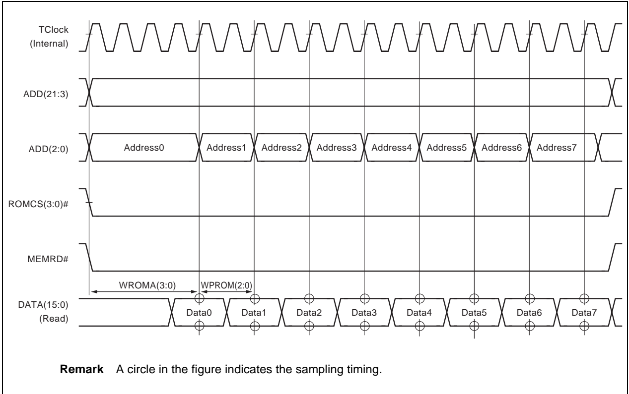
Figure 11-4. PageROM Read Cycle (WROMA(3:0) = 0011, WPROM(2:0) = 001)
