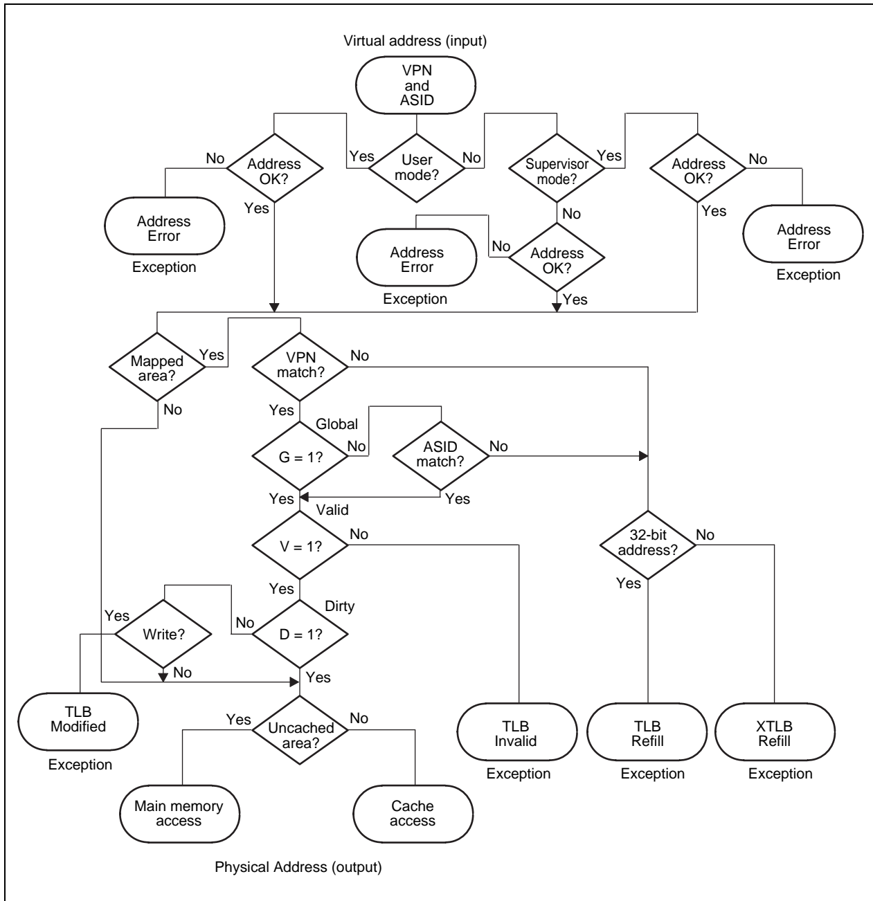
Figure 6-23. TLB Address Translation
