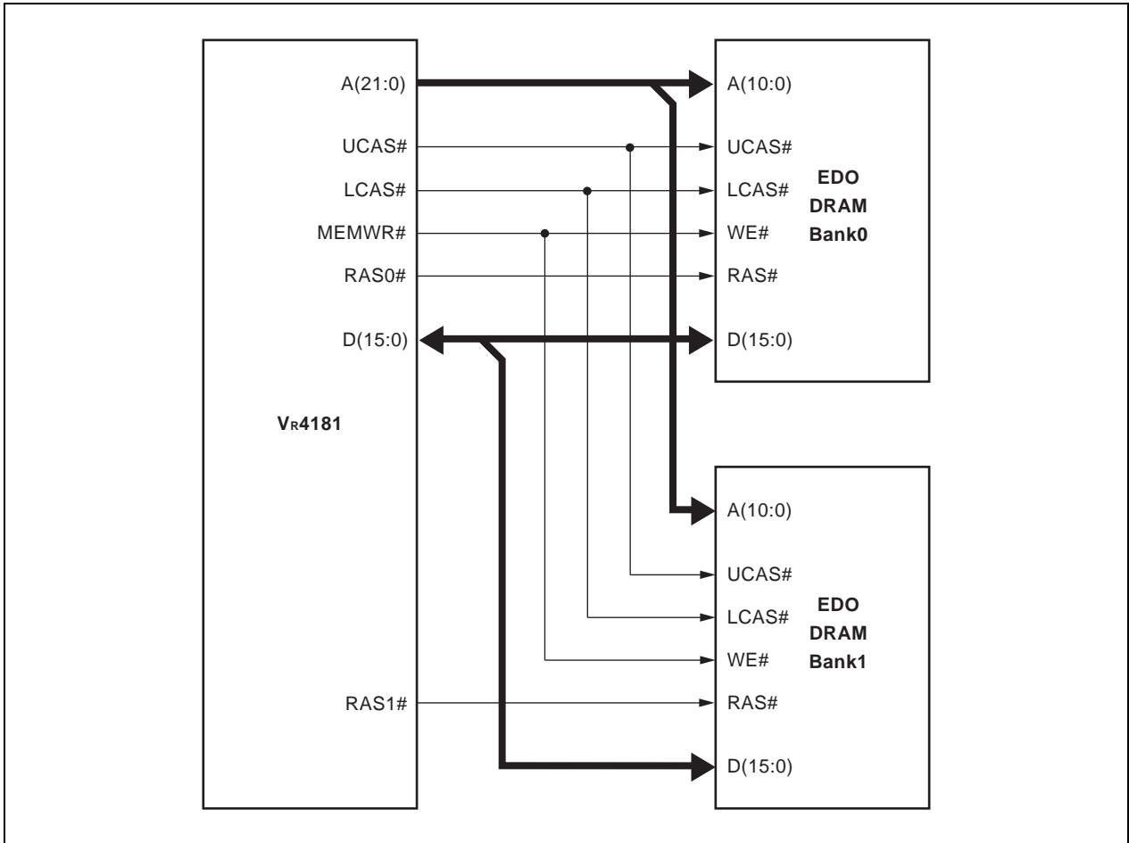
Figure 11-7. External EDO DRAM Configuration
