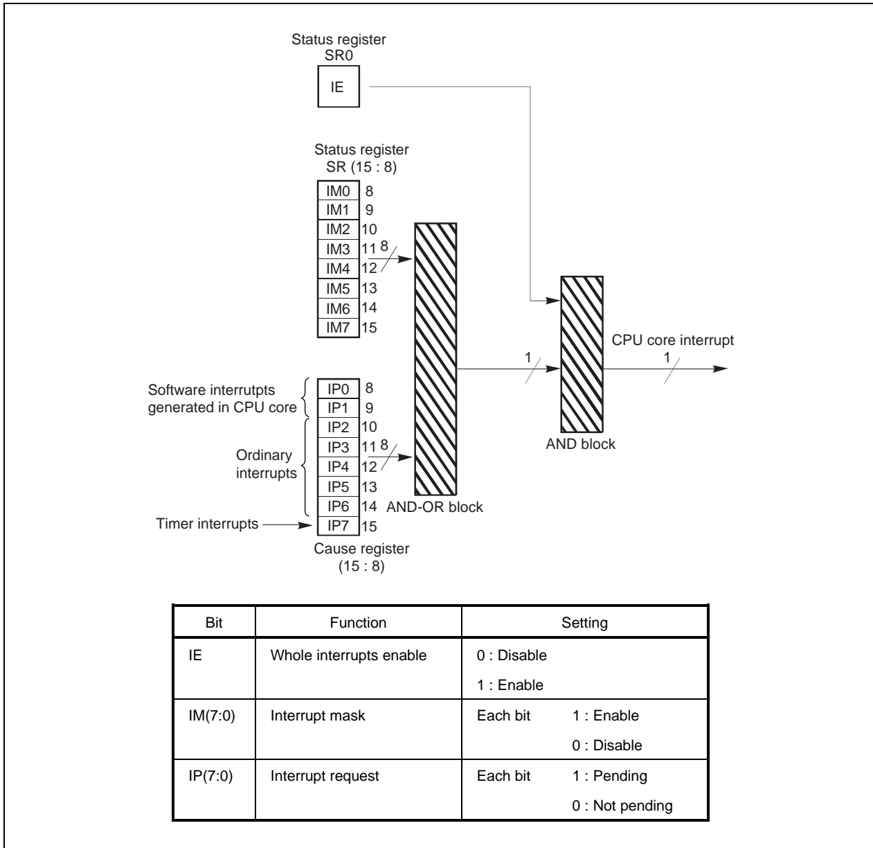
Figure 10-3. Masking of the Interrupt Request Signals
