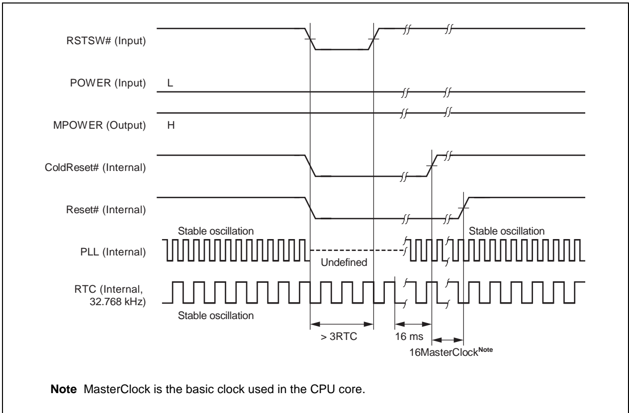
Figure 8-2. RSTSW
