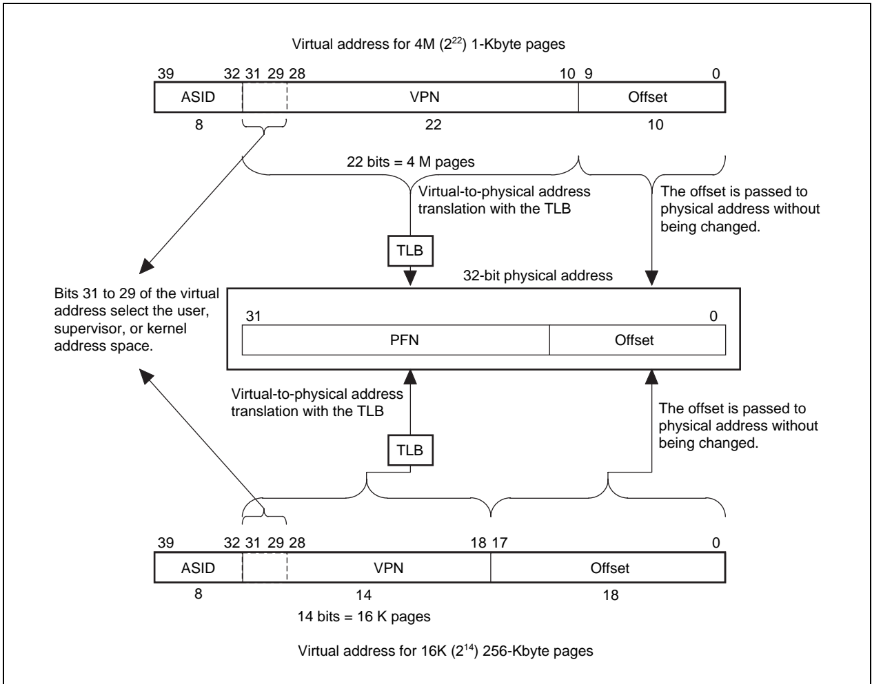
Figure 6-2. 32-bit Mode Virtual Address Translation
