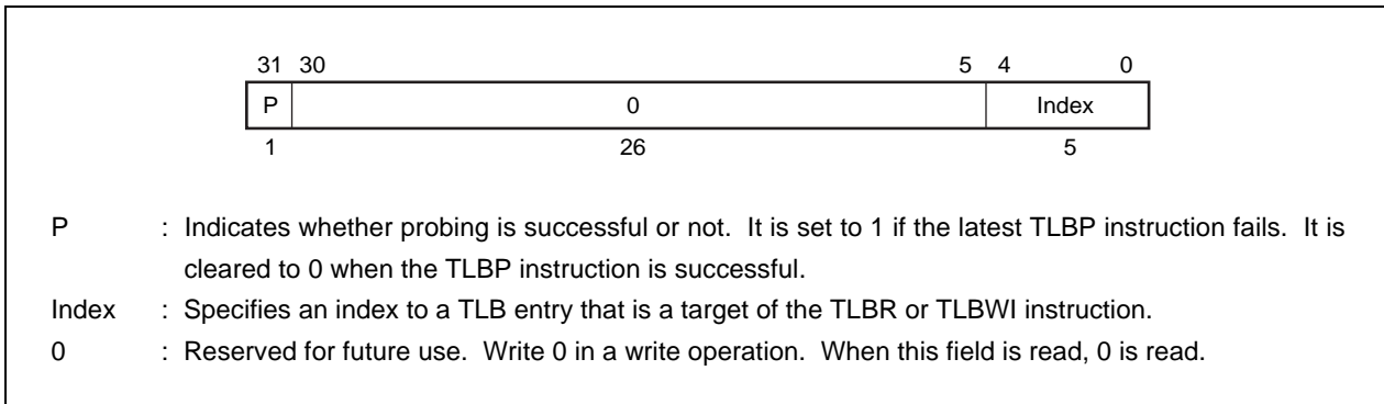
Figure 6-11. Index Register
