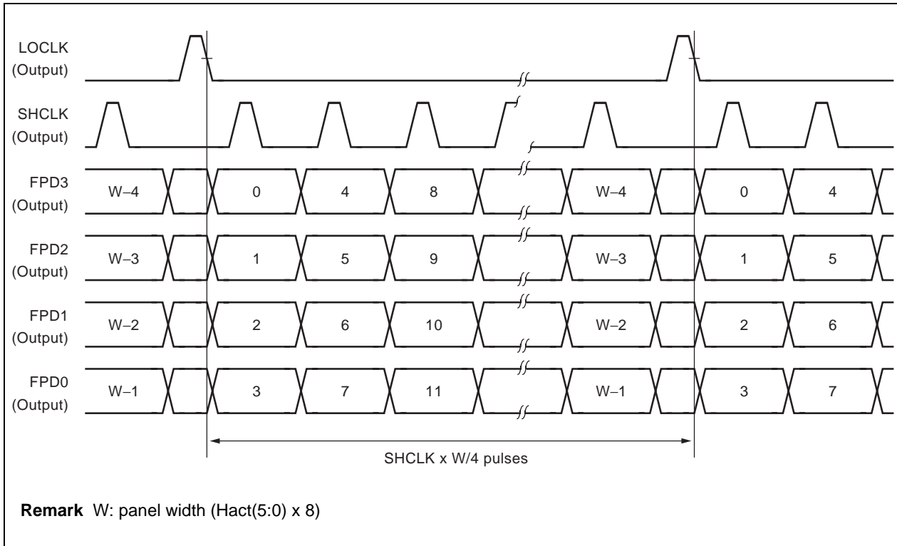
Figure 26-5. Monochrome Panel
