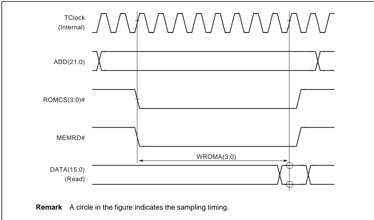
Figure 11-5. Flash Memory Read Cycle (WROMA(3:0) = 0111)
