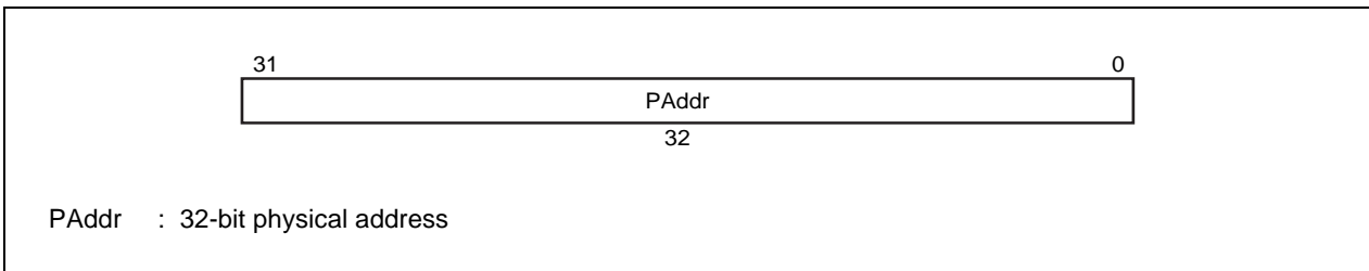
Figure 6-20. LLAddr Register
