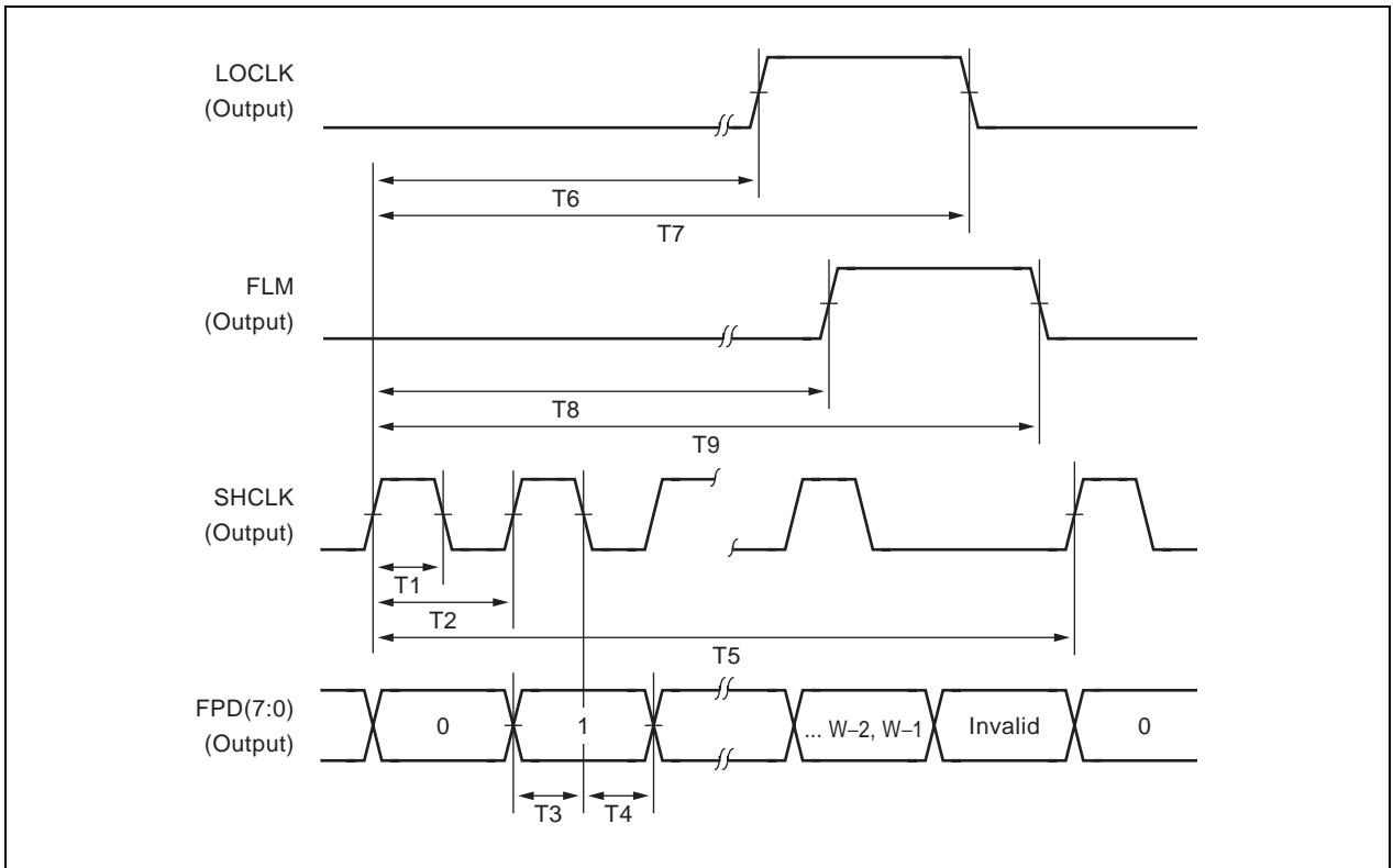
Figure 26-9. LCD Timing Parameters
