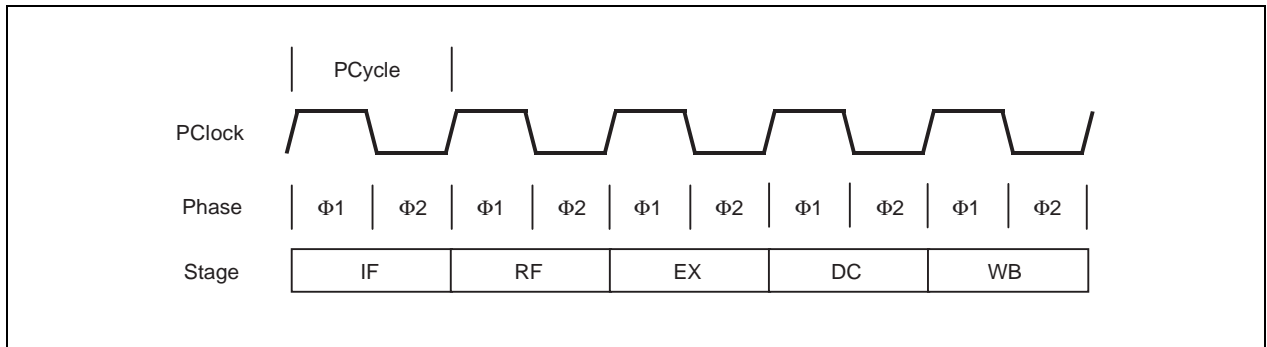
Figure 5-1. Pipeline Stages
