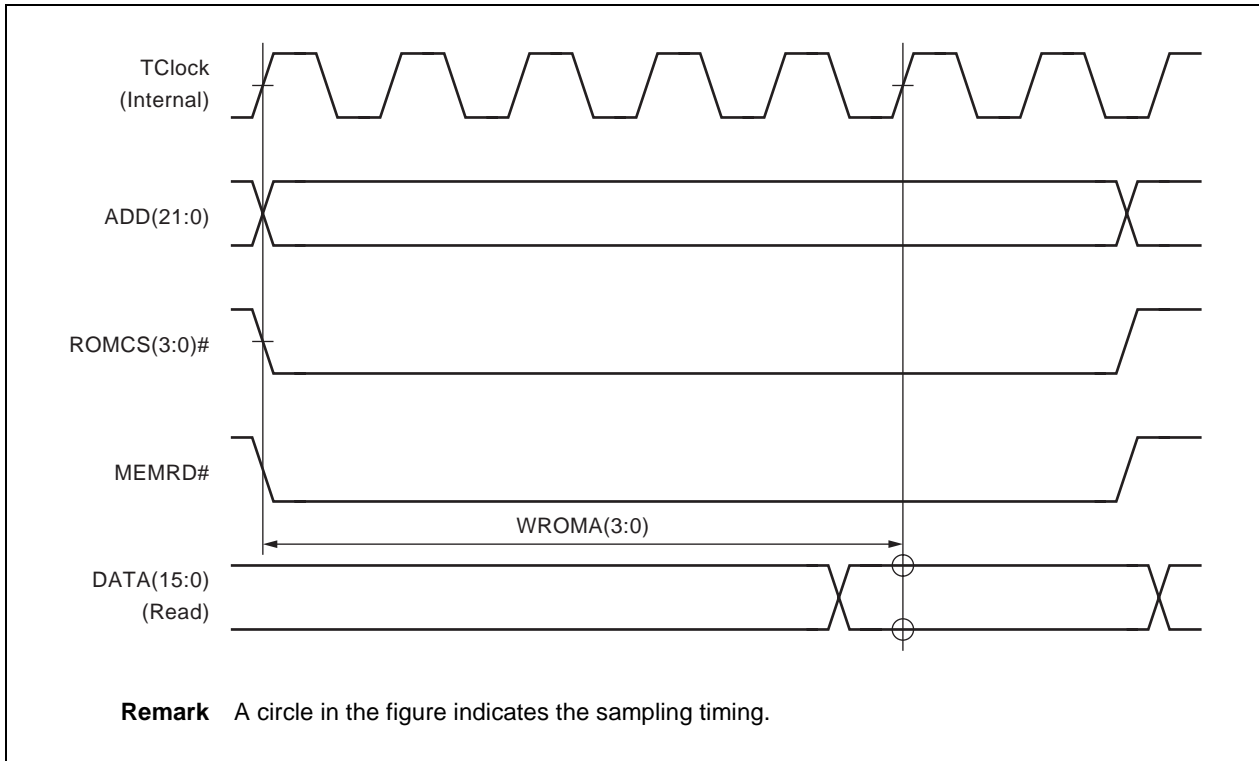
Figure 11-3. Ordinary ROM Read Cycle (WROMA(3:0) = 0100)
