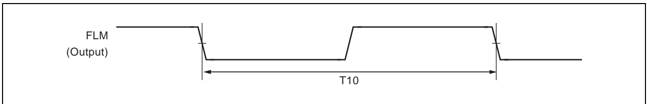
Figure 26-10. FLM Period
