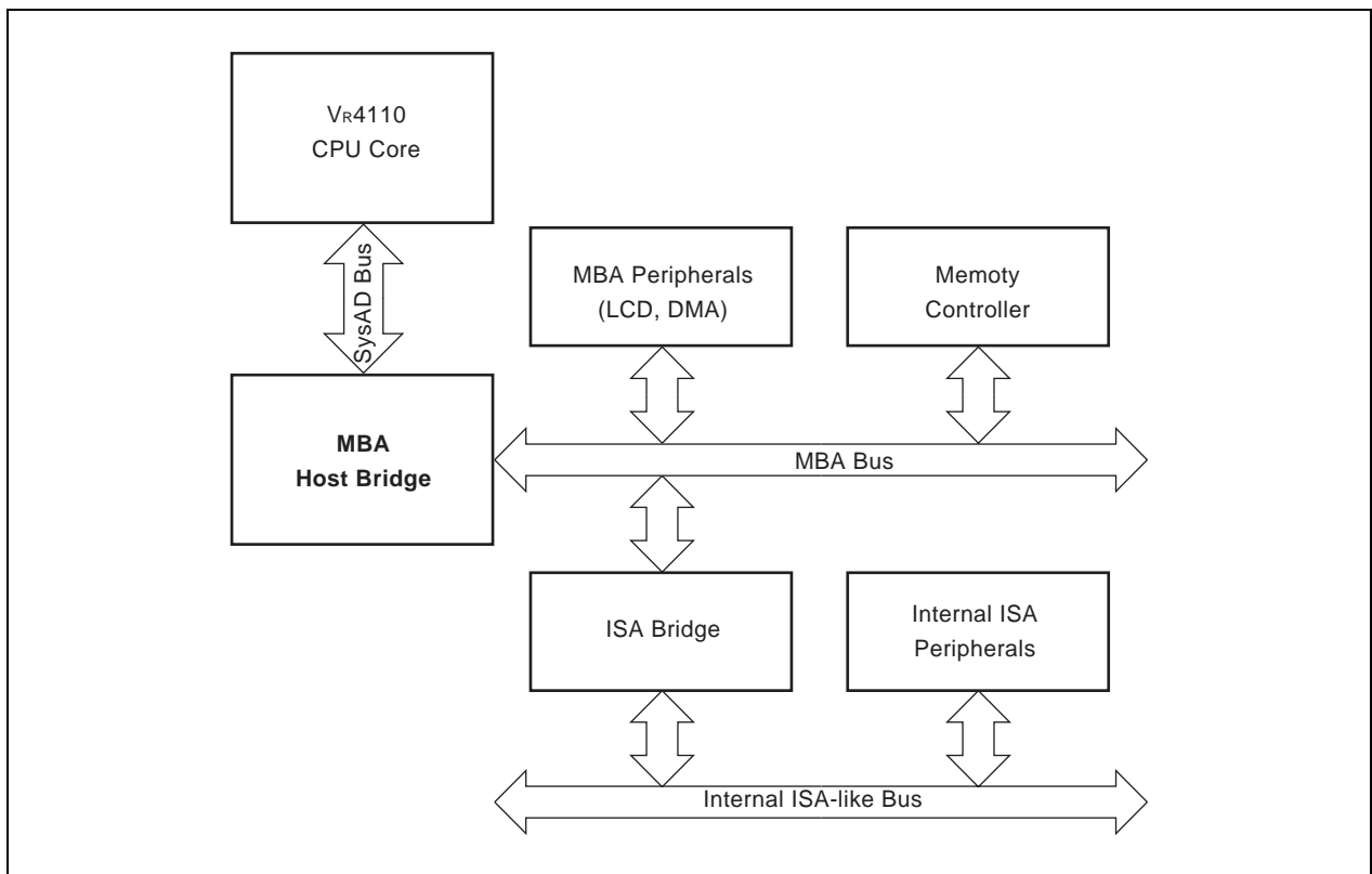
Figure 11-1. VR4181 Internal Bus Structure
