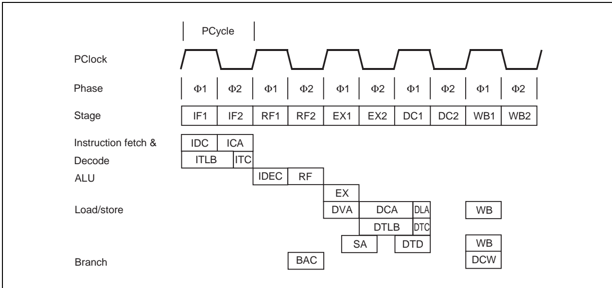
Figure 5-3. Pipeline Activities
