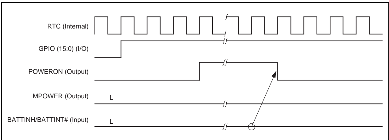
Figure 15-7. Activation via GPIO Activation Interrupt (BATTINH = L)
