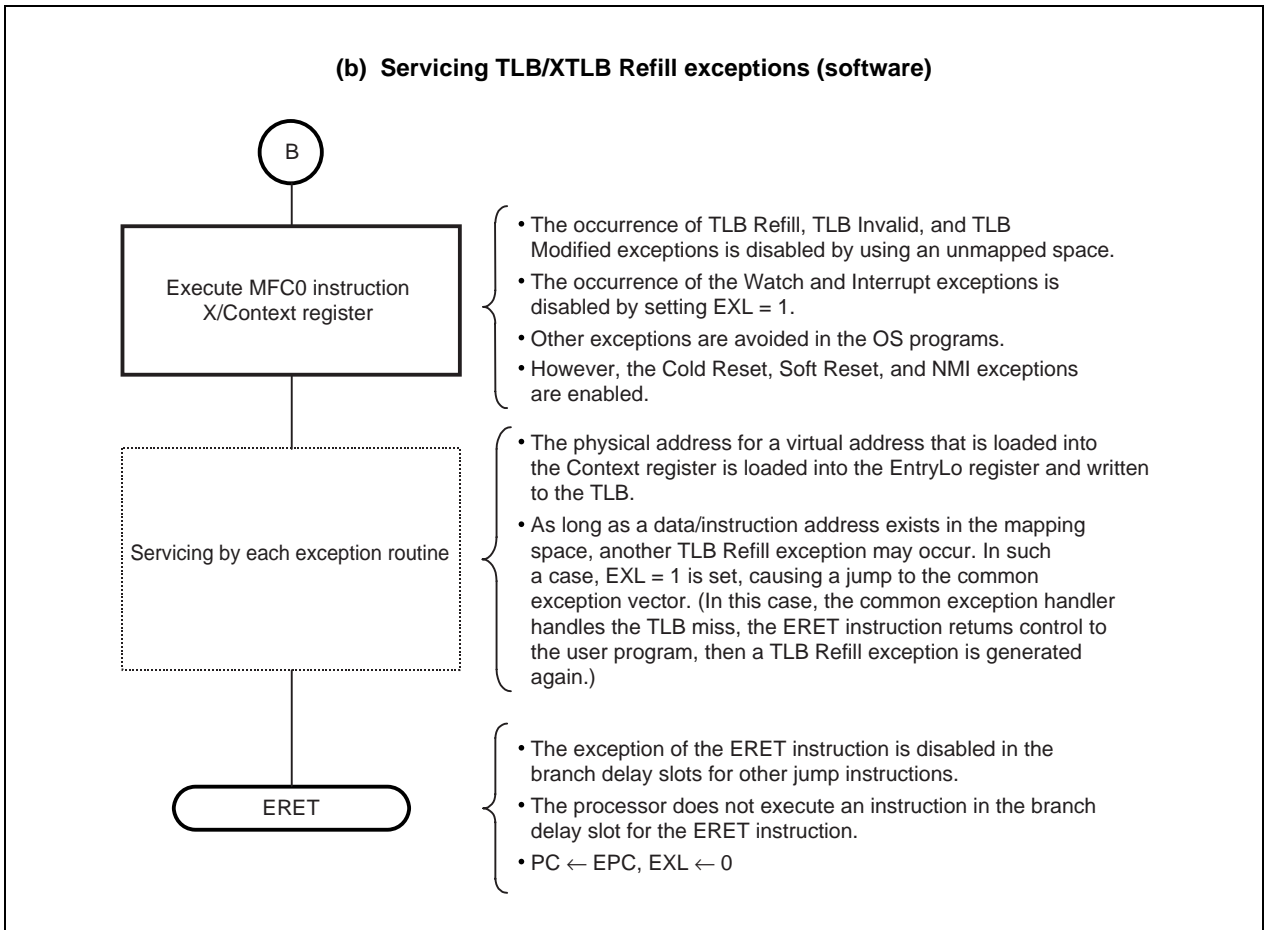
Figure 7-18. TLB/XTLB Refill Exception Handling (2/2)
