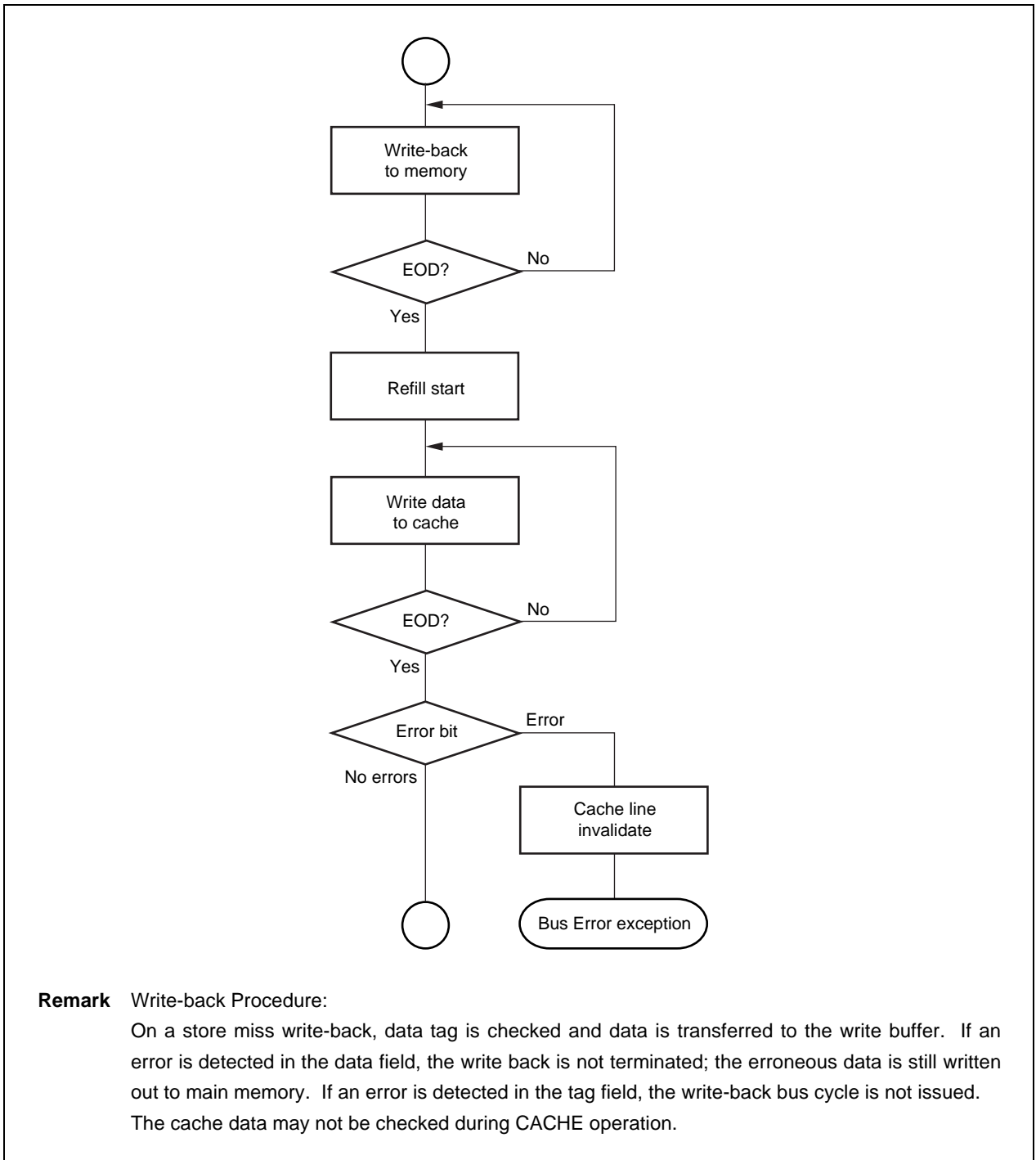
Figure 9-22. Writeback &amp; Refill Flow
