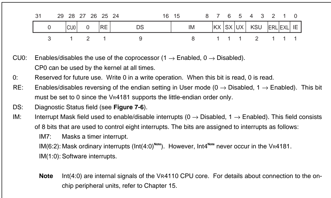
Figure 7-5. Status Register Format (1/2)
