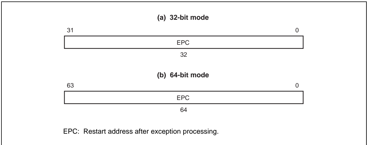
Figure 7-8. EPC Register Format (When MIPS16 ISA Is Disabled)
