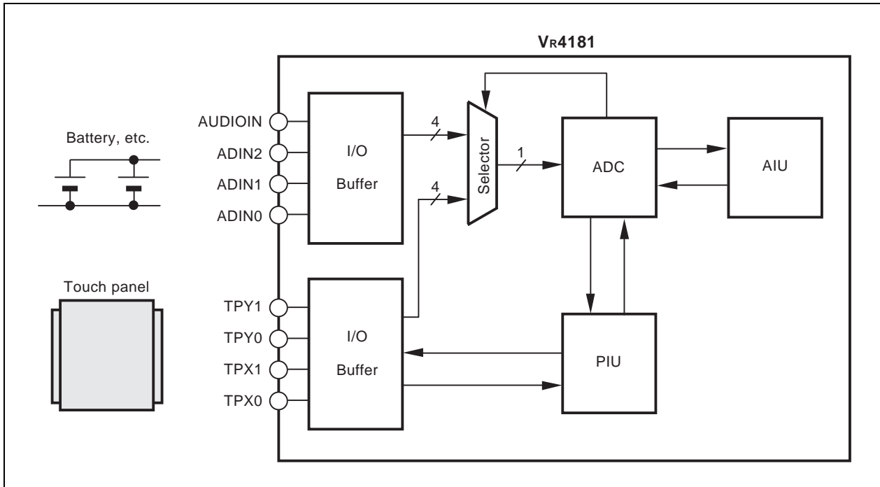
Figure 19-1. PIU Peripheral Block Diagram
