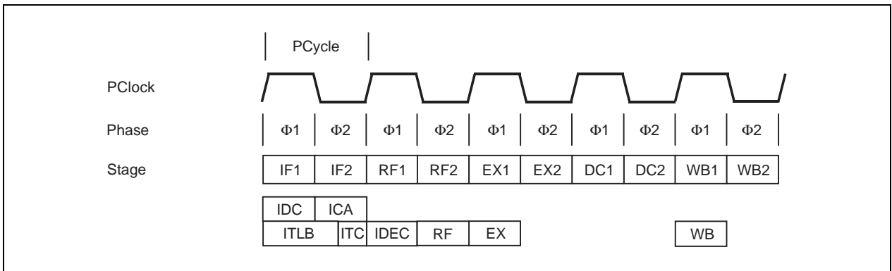
Figure 5-5. Add Instruction Pipeline Activities
