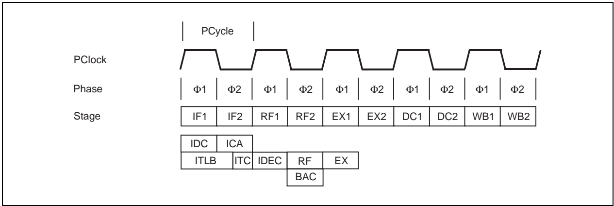
Figure 5-7. BEQ Instruction Pipeline Activities
