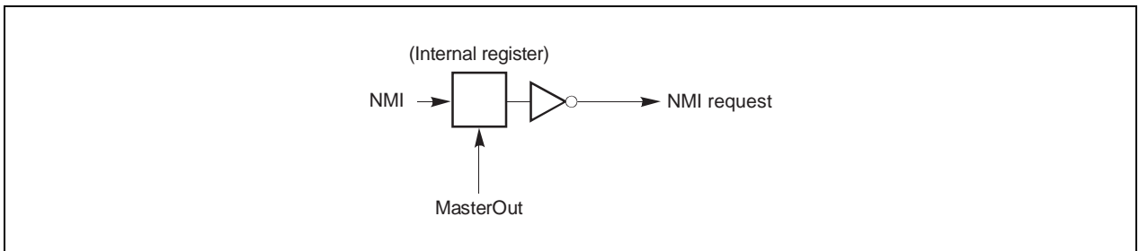
Figure 10-1. Non-maskable Interrupt Signal
