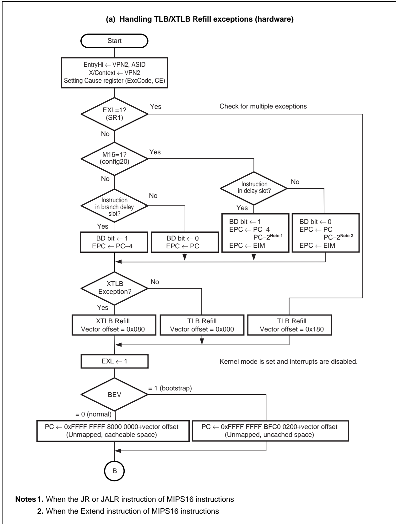
Figure 7-18. TLB/XTLB Refill Exception Handling (1/2)
