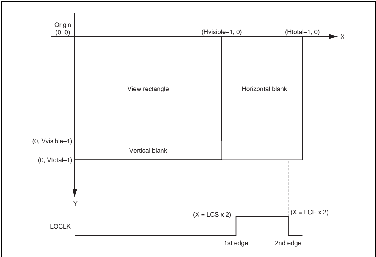
Figure 26-3. Position of Load Clock, LOCLK
