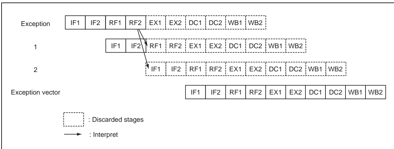
Figure 5-12. Exception Detection
