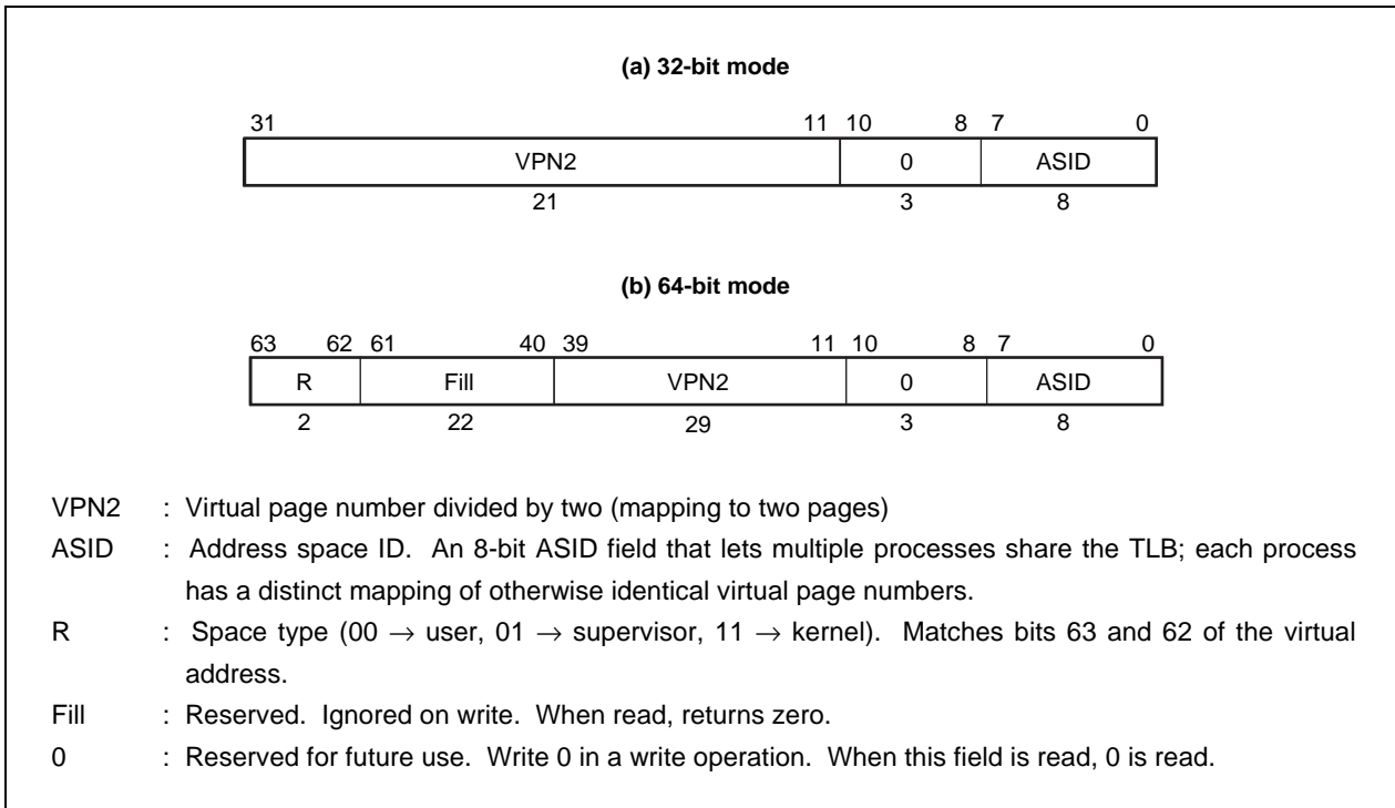
Figure 6-17. EntryHi Register
