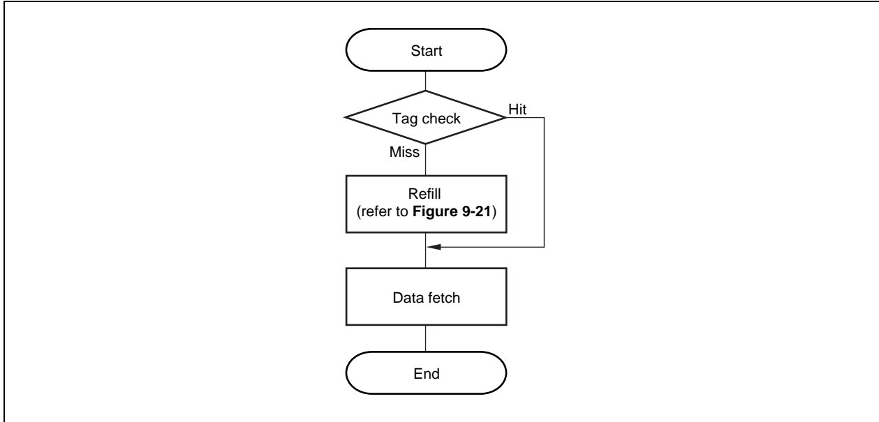
Figure 9-9. Data Check Flow on Load Operations
