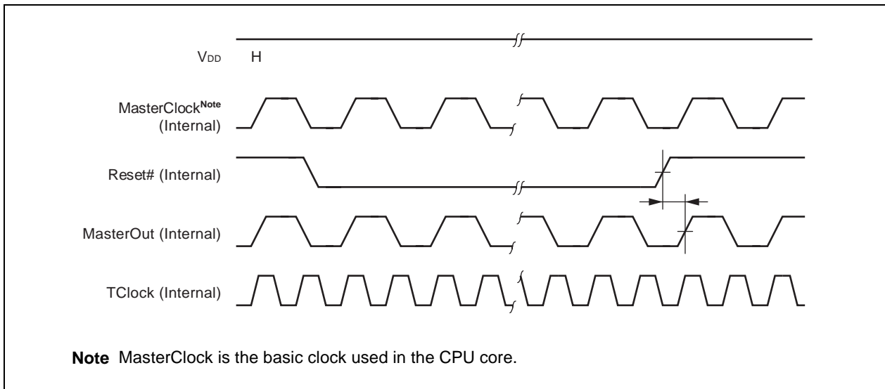
Figure 8-9. Soft Reset
