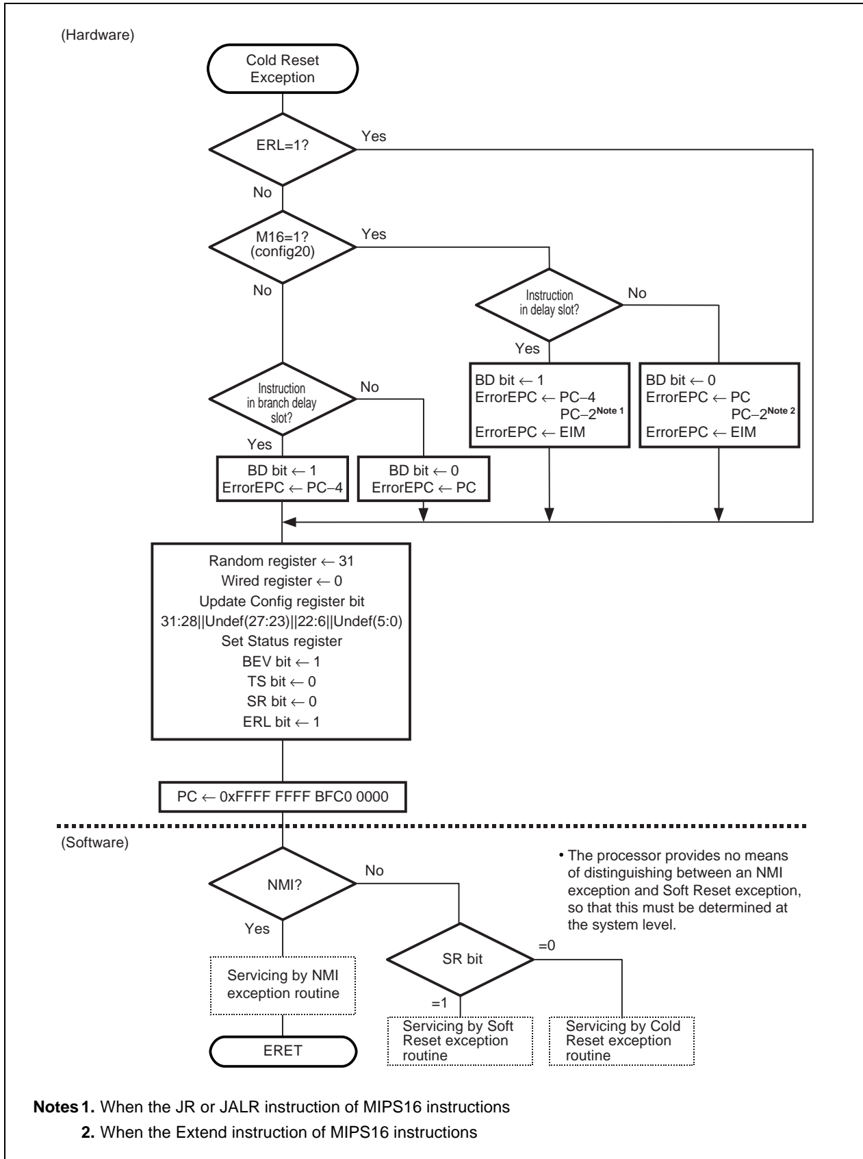
Figure 7-19. Cold Reset Exception Handling
