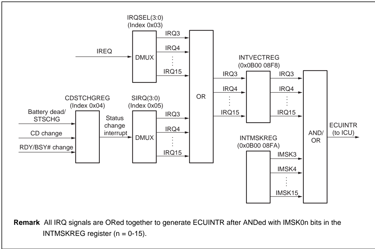
Figure 22-1. CompactFlash Interrupt Logic
