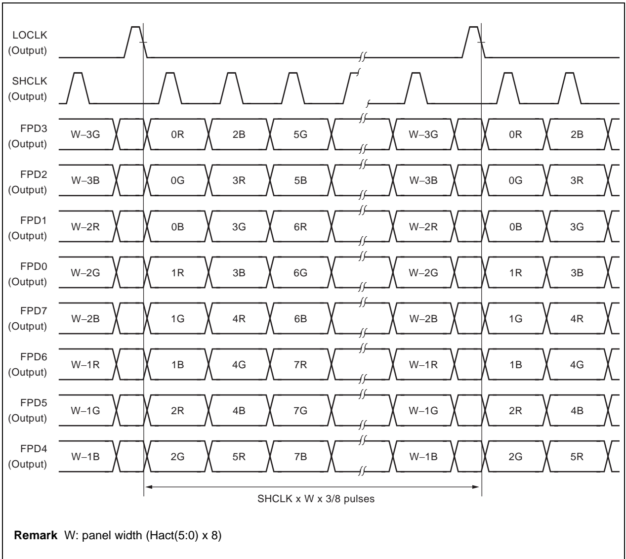
Figure 26-6. Color Panel in 8-bit Data Bus
