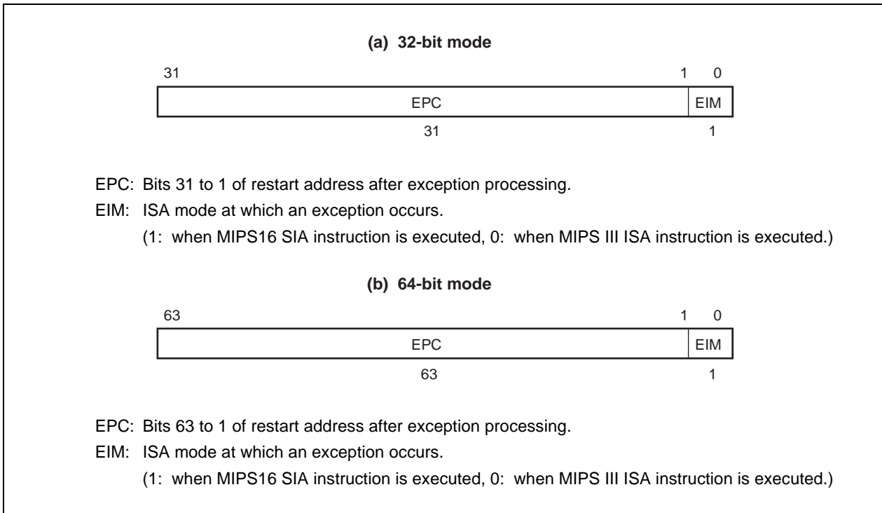
Figure 7-9. EPC Register Format (When MIPS16 ISA Is Enabled)
