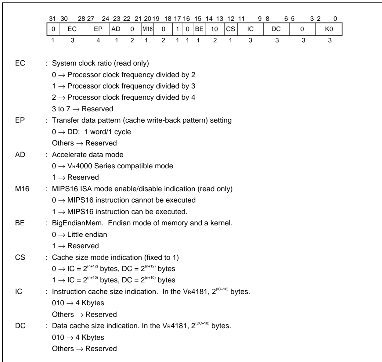
Figure 6-19. Config Register Format (1/2)
