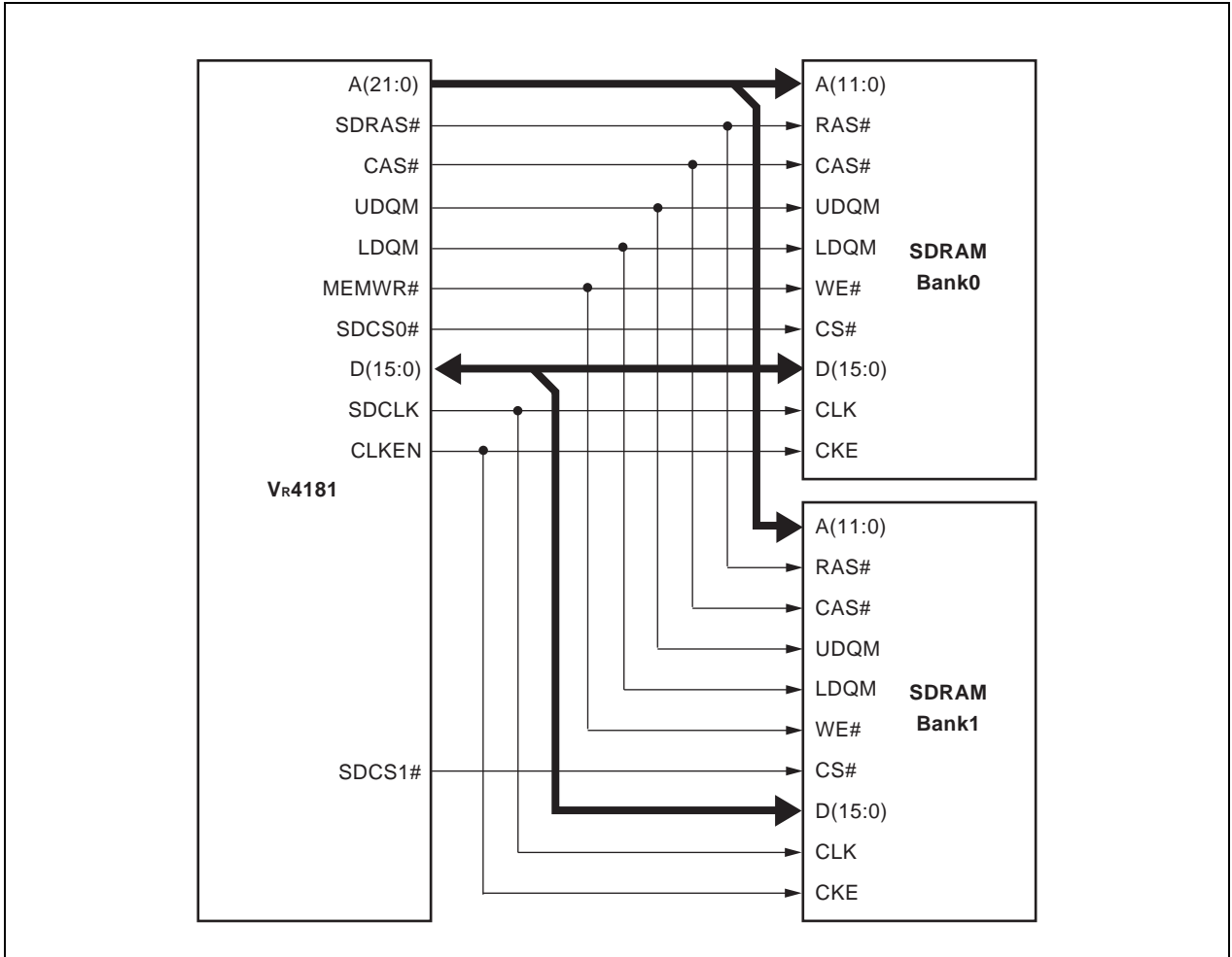
Figure 11-8. SDRAM Configuration
