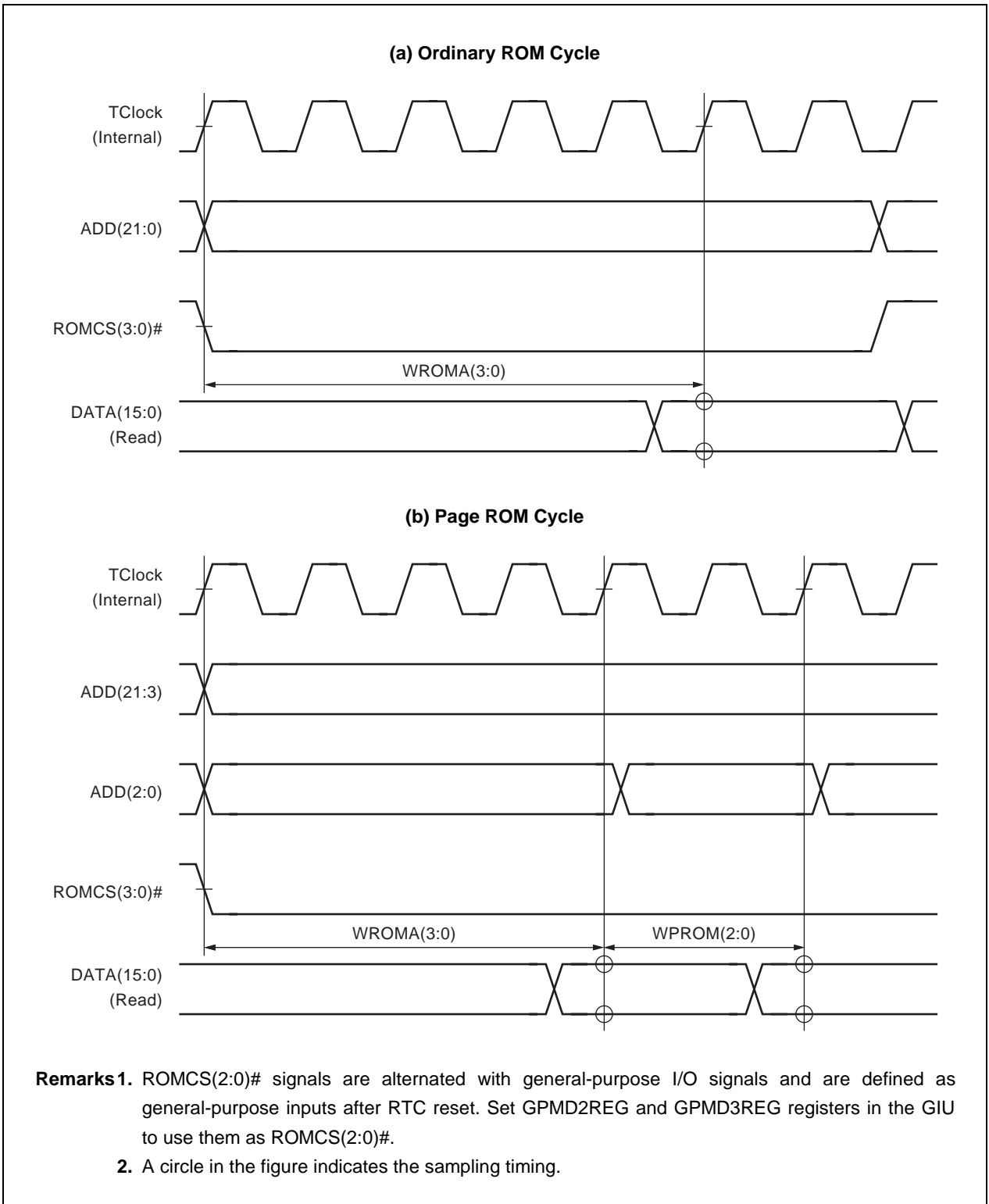
Figure 11-2. ROM Read Cycle
