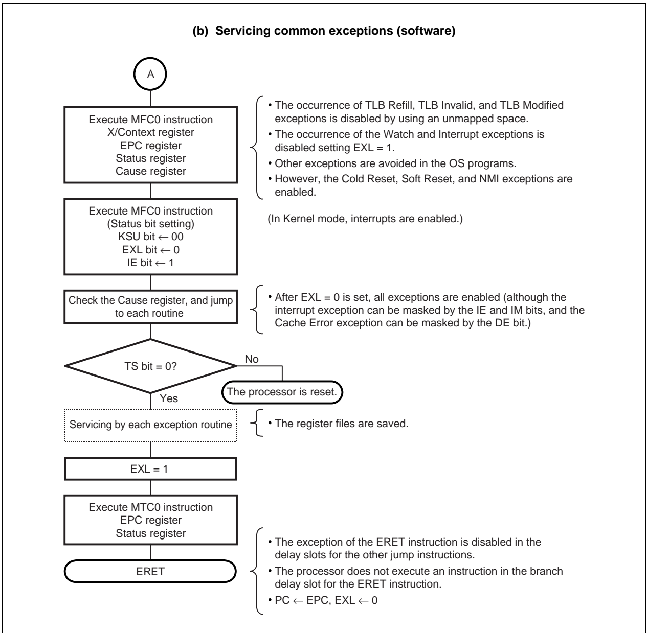
Figure 7-17. Common Exception Handling (2/2)
