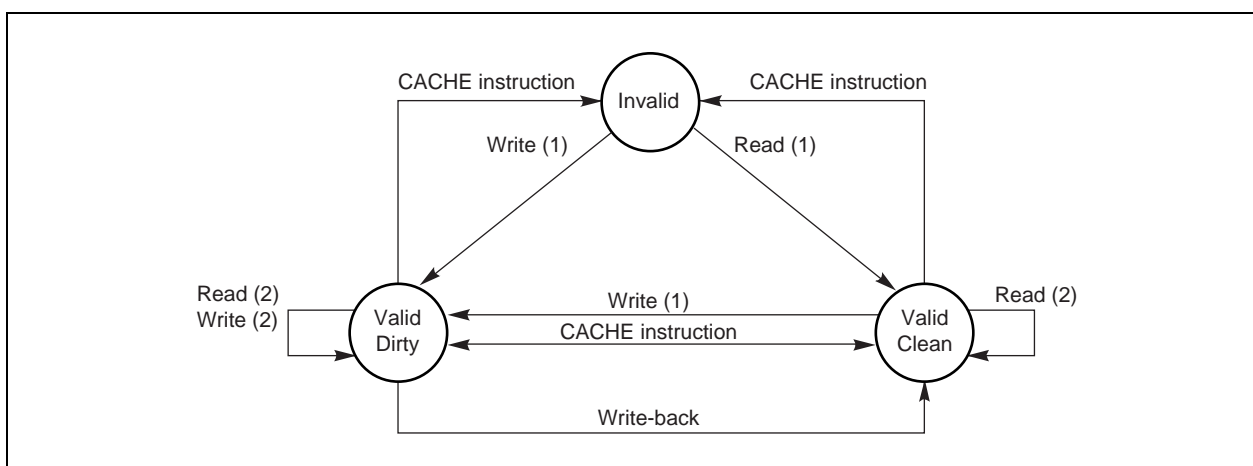
Figure 9-6. Data Cache State Diagram
