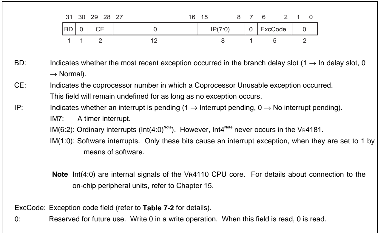
Figure 7-7. Cause Register Format
