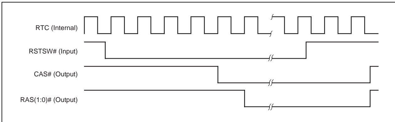
Figure 15-1. EDO DRAM Signals on RSTSW Reset (SDRAM bit = 0)
