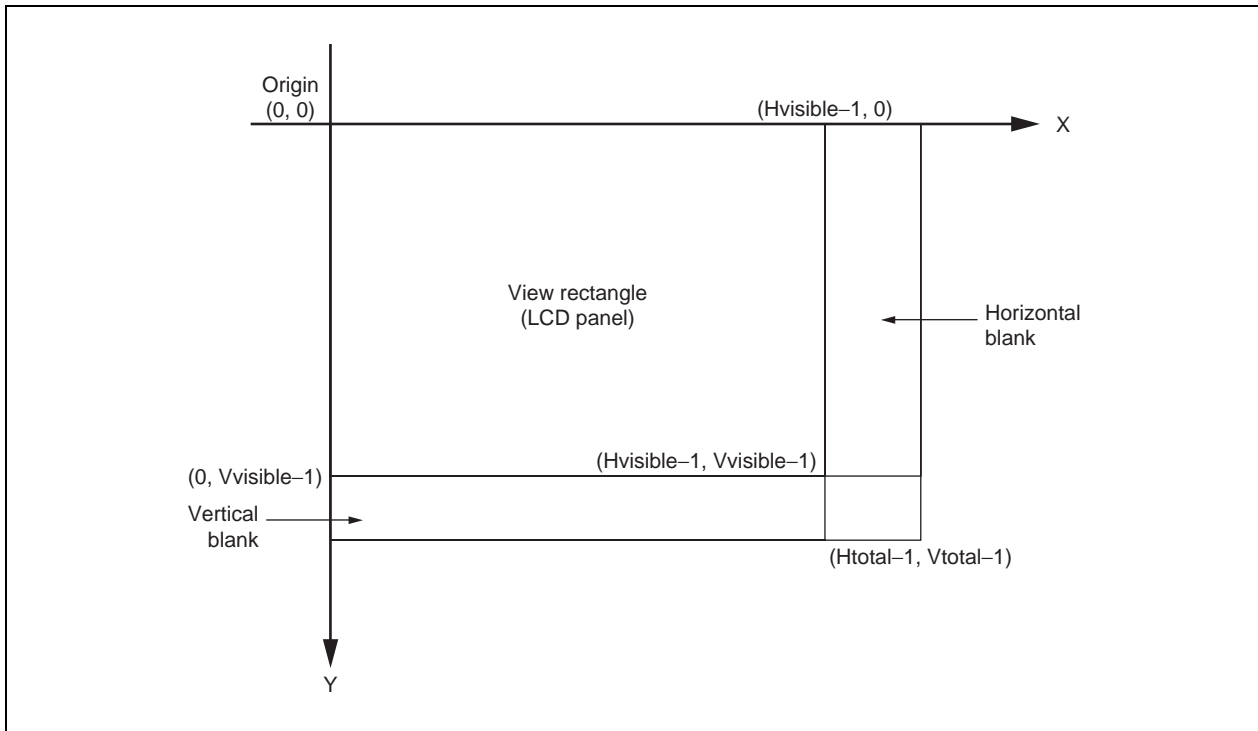
Figure 26-2. View Rectangle and Horizontal/Vertical Blank
