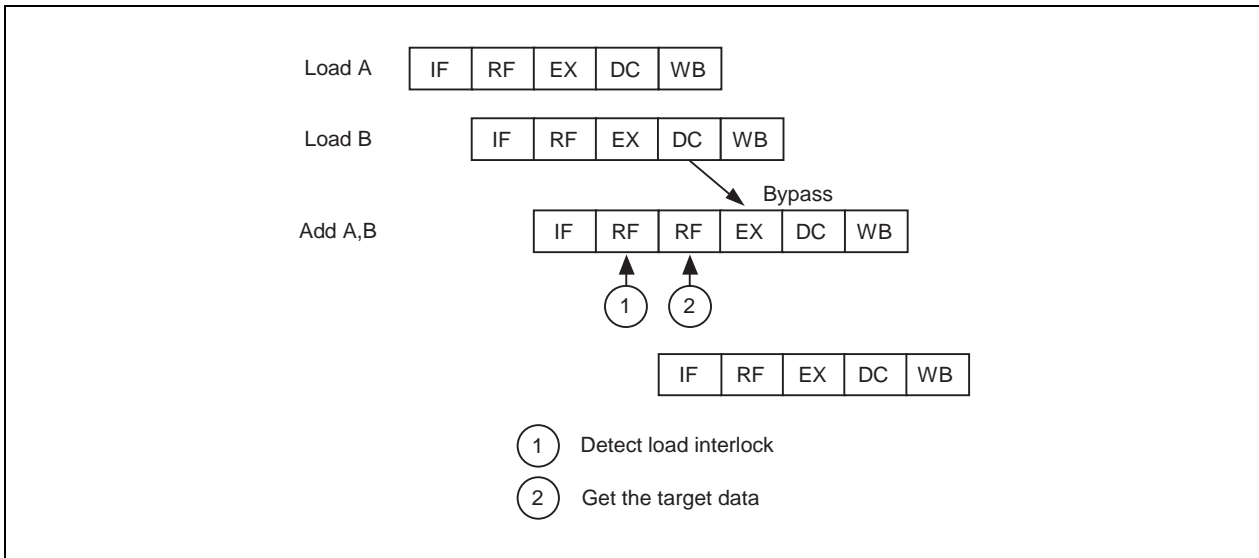
Figure 5-15. Load Data Interlock
