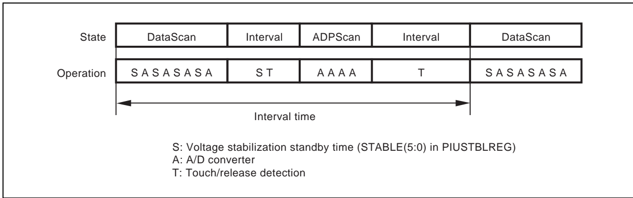
Figure 19-5. Interval Times and States
