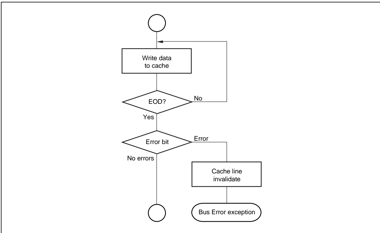
Figure 9-21. Refill Flow
