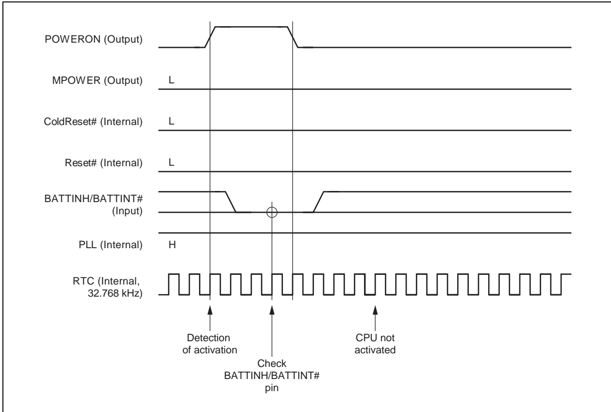
Figure 8-7. V R 4181 Activation Sequence (when activation is NG)
