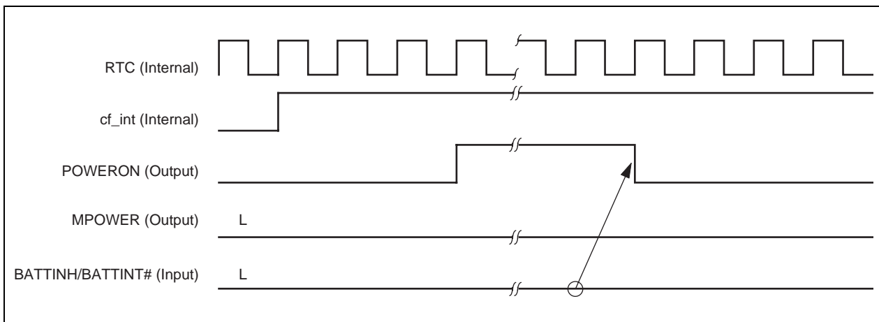
Figure 15-5. Activation via CompactFlash Interrupt Request (BATTINH = L)
