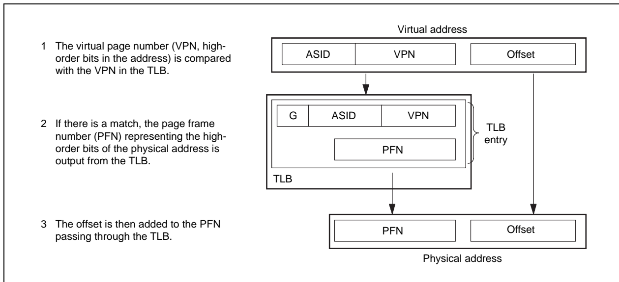
Figure 6-1. Virtual-to-Physical Address Translation
