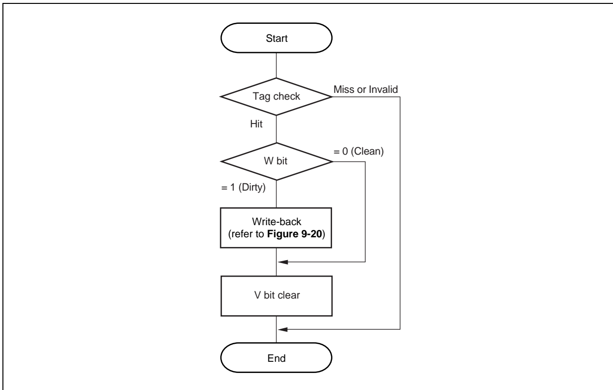
Figure 9-17. Data Check Flow on Hit_Writeback_Invalidate Operations
