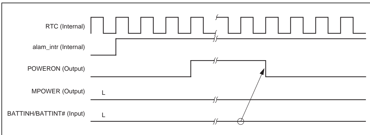
Figure 15-11. Activation via Alarm Interrupt (BATTINH = L)
