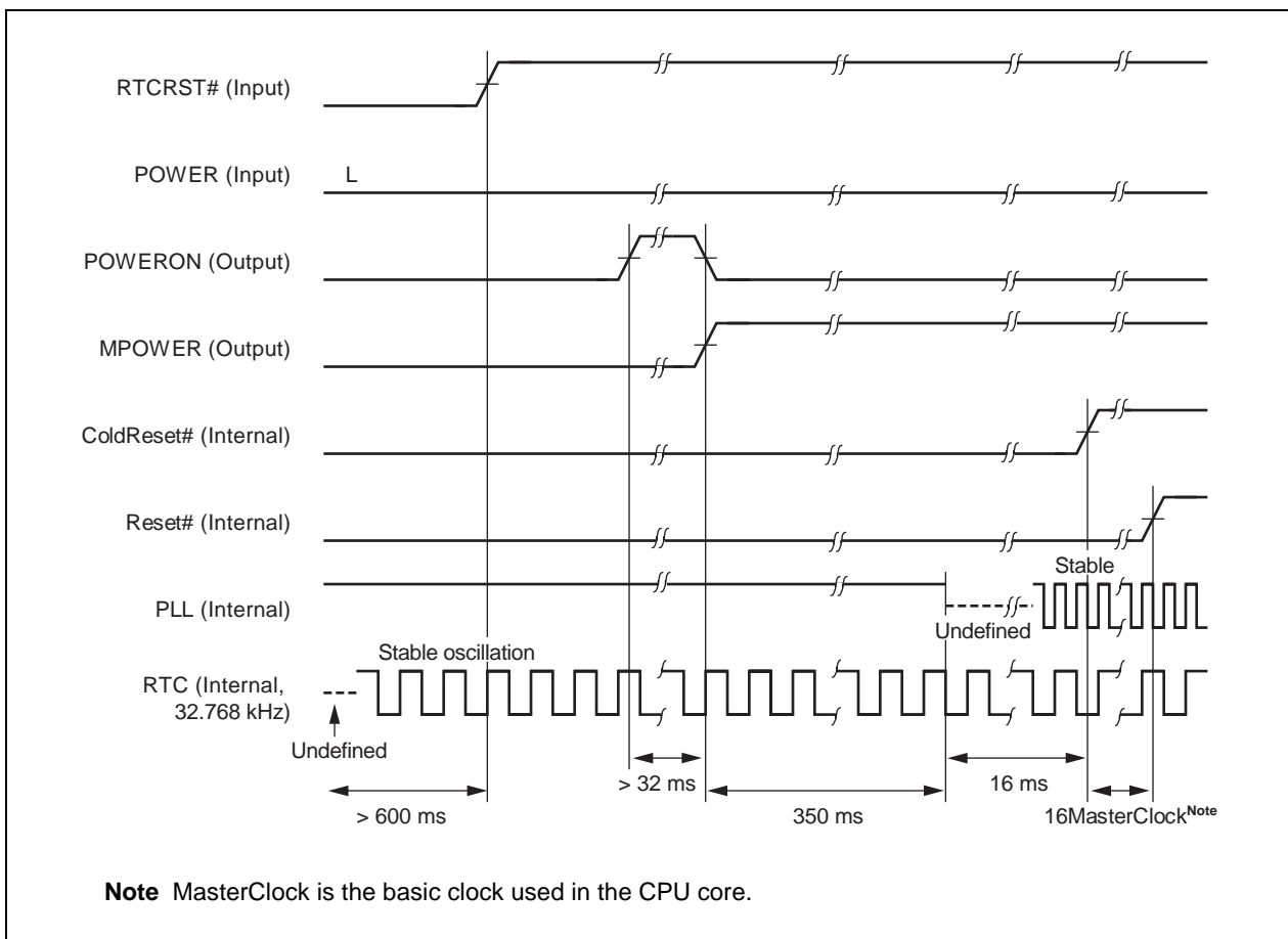
Figure 8-1. RTC Reset
