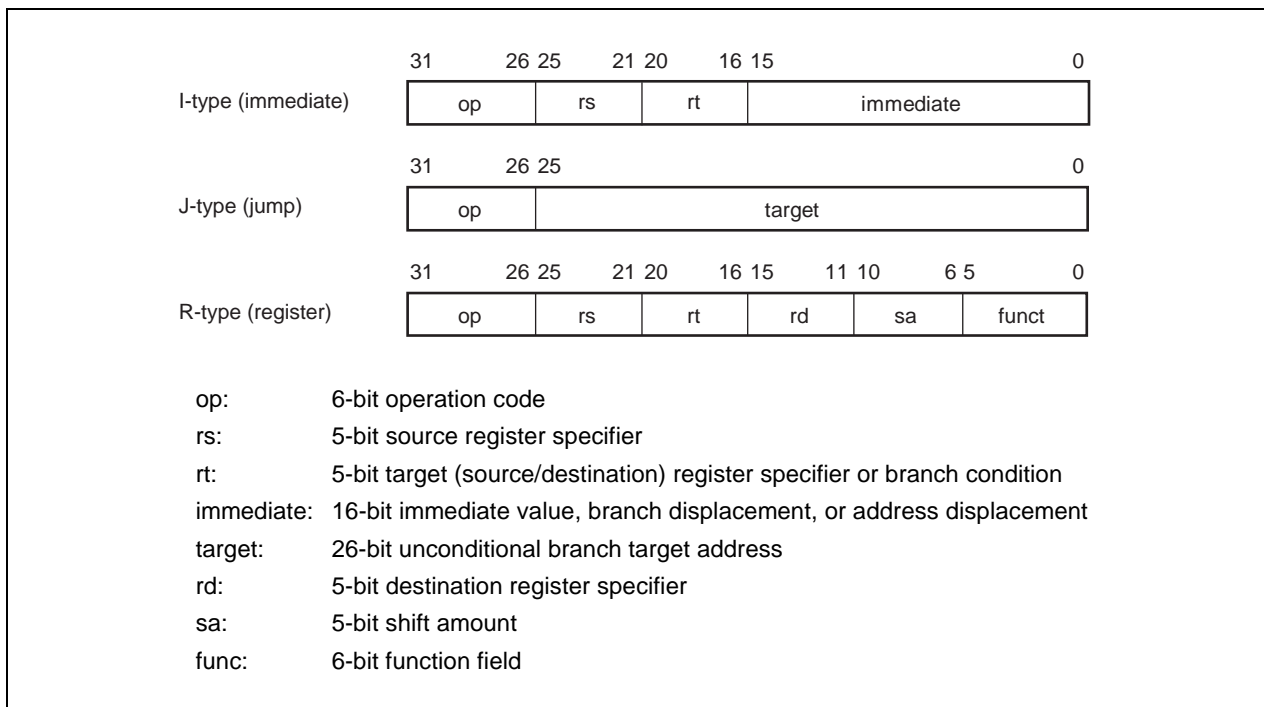
Figure 3-1. MIPS III ISA CPU Instruction Formats
