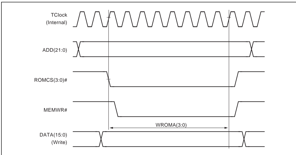
Figure 11-6. Flash Memory Write Cycle (WROMA(3:0) = 0111)
