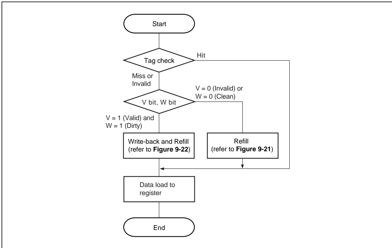
Figure 9-9. Data Check Flow on Load Operations
