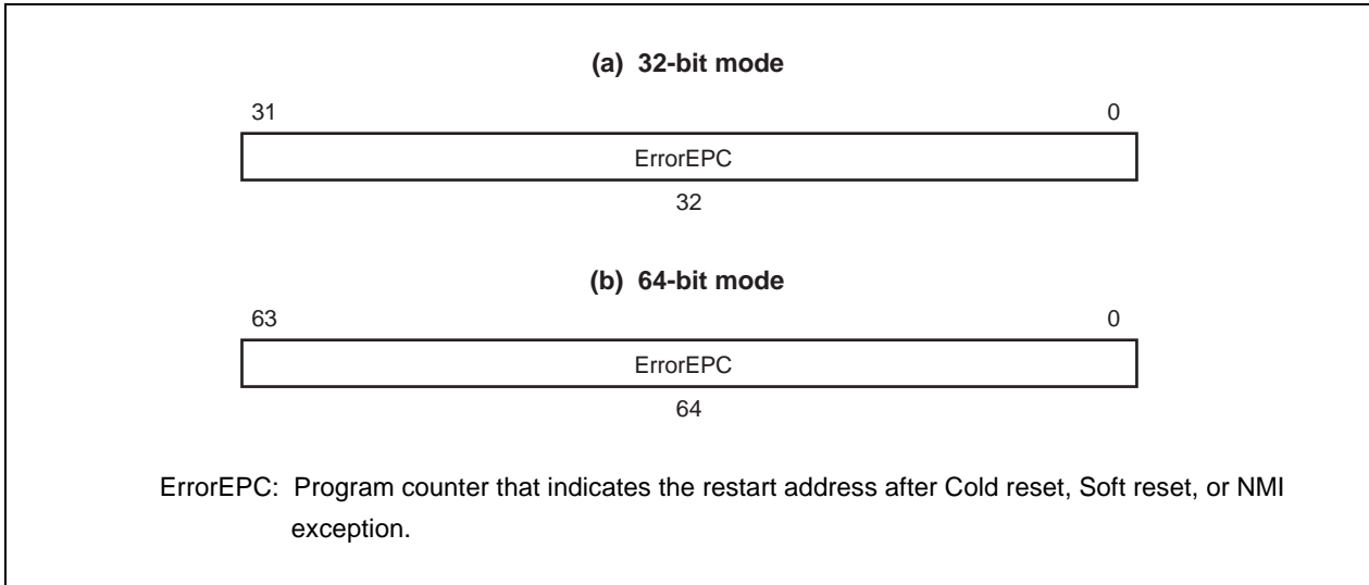
Figure 7-16. ErrorEPC Register Format (When MIPS16 ISA Is Enabled)
