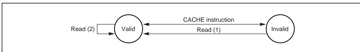
Figure 9-7. Instruction Cache State Diagram
