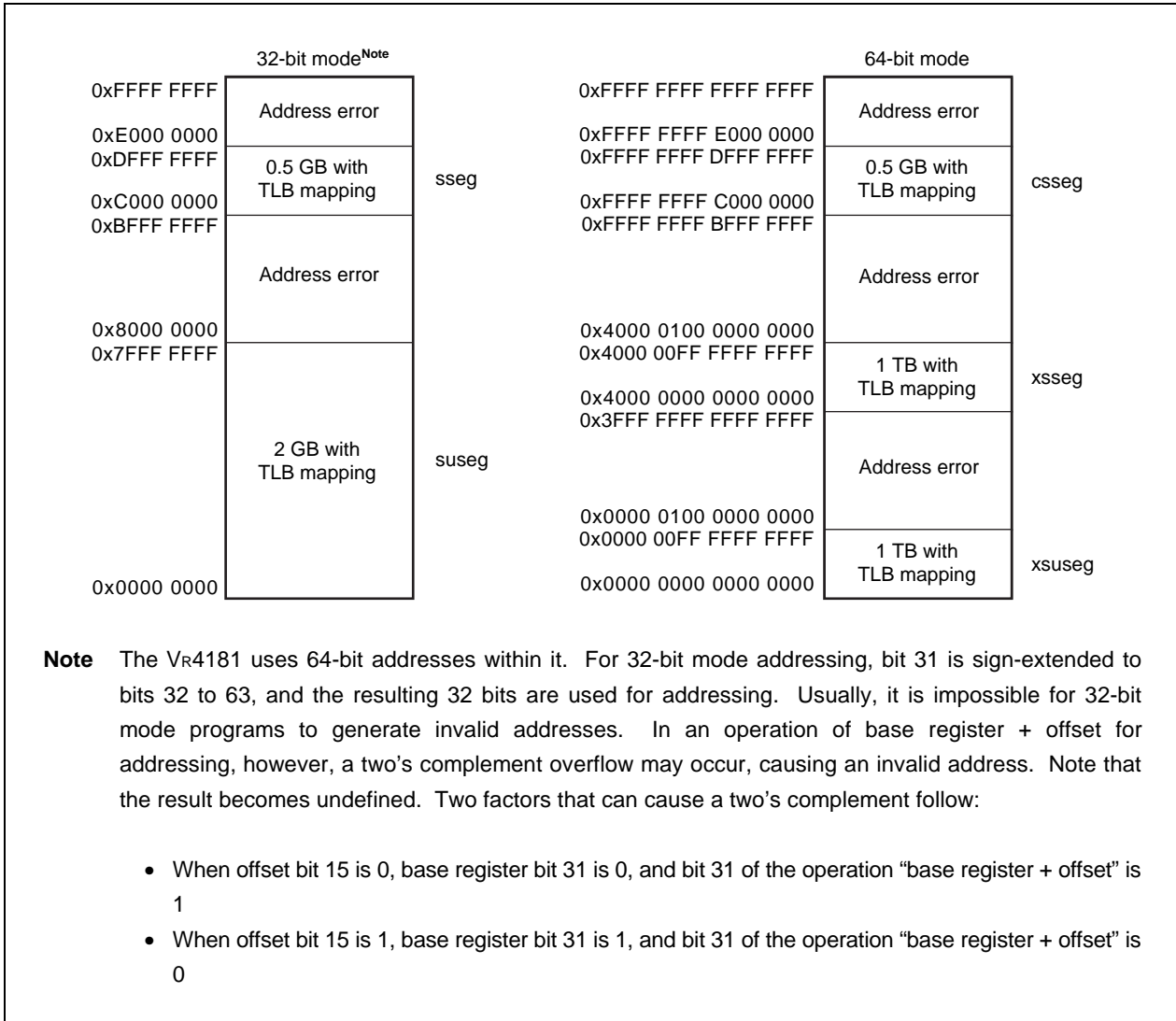
Figure 6-5. Supervisor Mode Address Space
