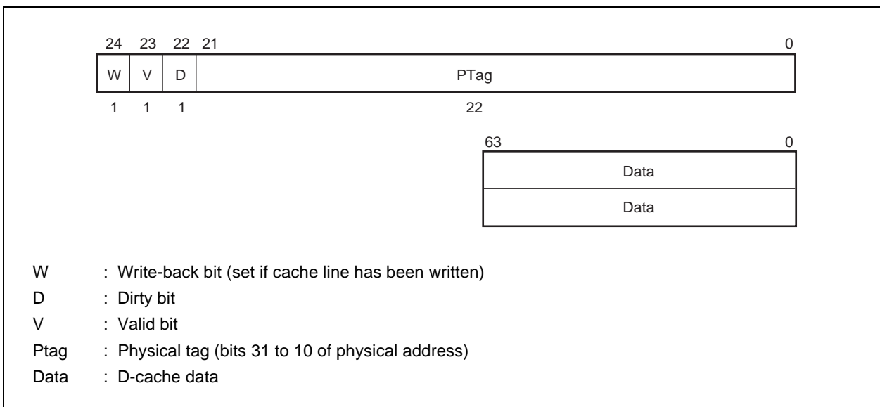
Figure 9-4. Data Cache Line Format
