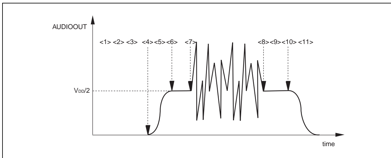
Figure 20-1. Speaker Output and AUDIOOUT Pin
