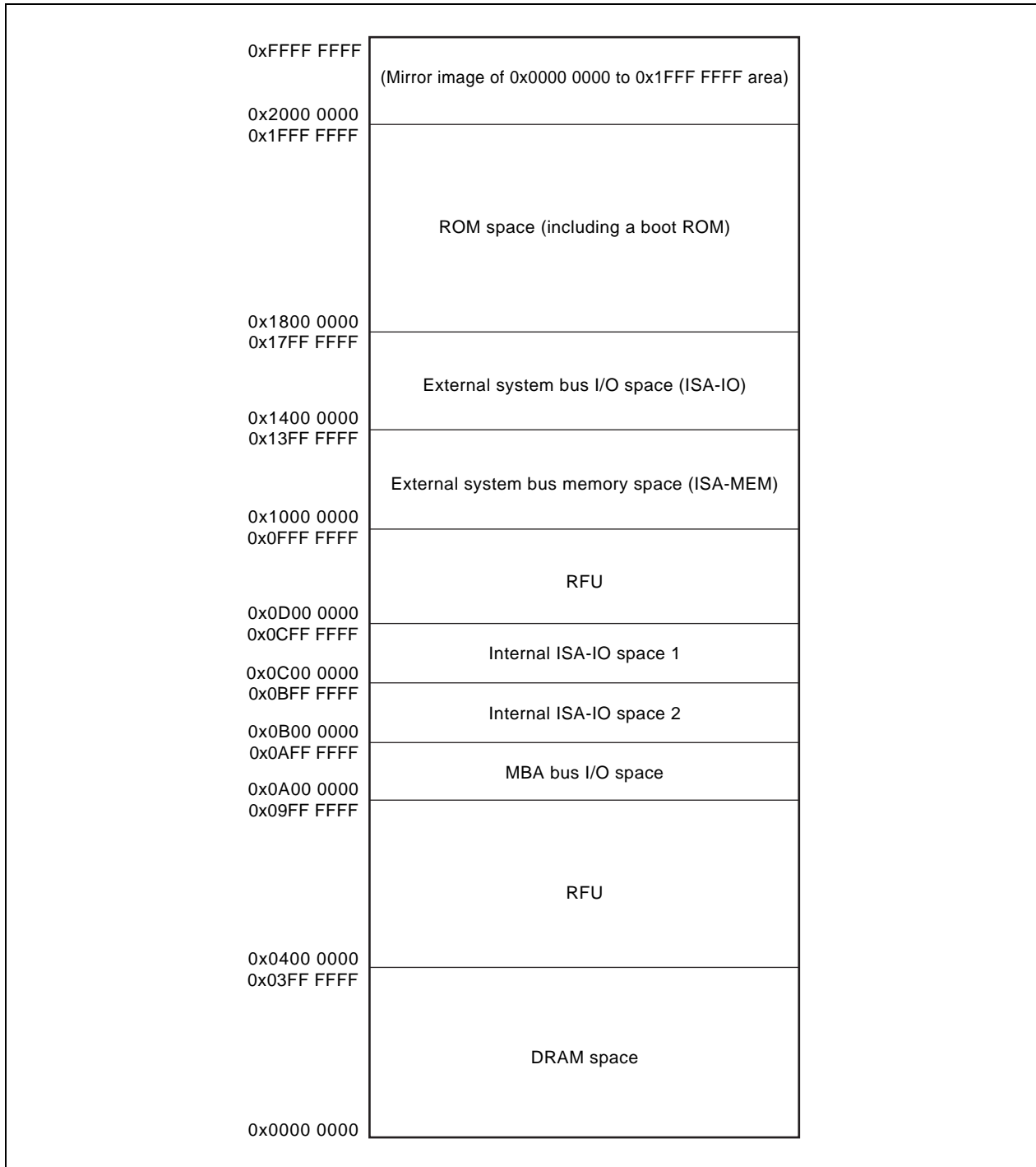
Figure 6-8. VR4181 Physical Address Space
