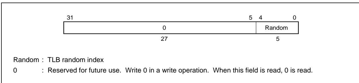
Figure 6-12. Random Register
