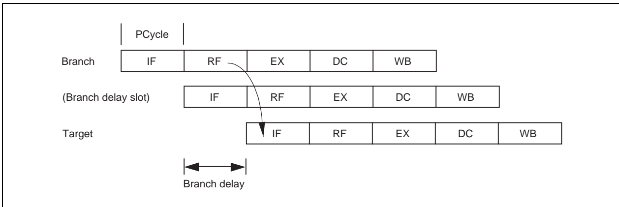
Figure 5-4. Branch Delay
