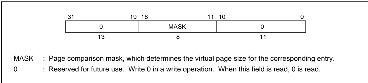
Figure 6-14. Page Mask Register
