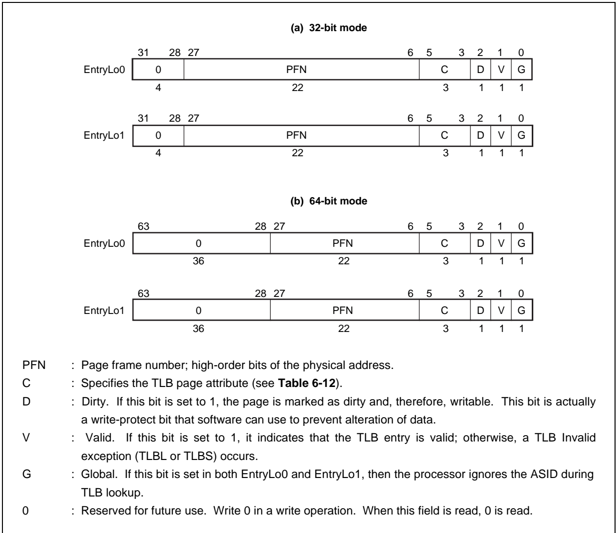
Figure 6-13. EntryLo0 and EntryLo1 Registers
