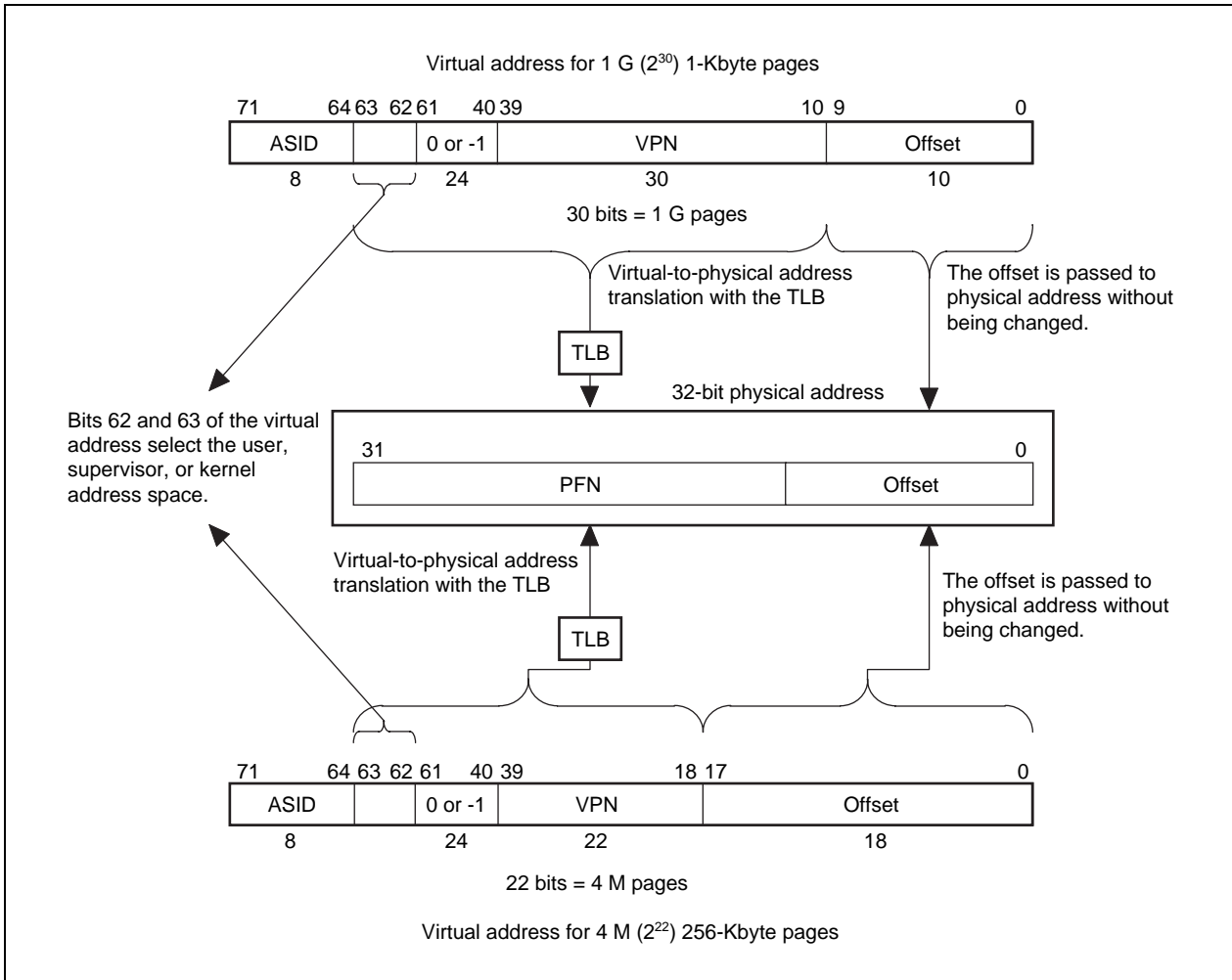
Figure 6-3. 64-bit Mode Virtual Address Translation
