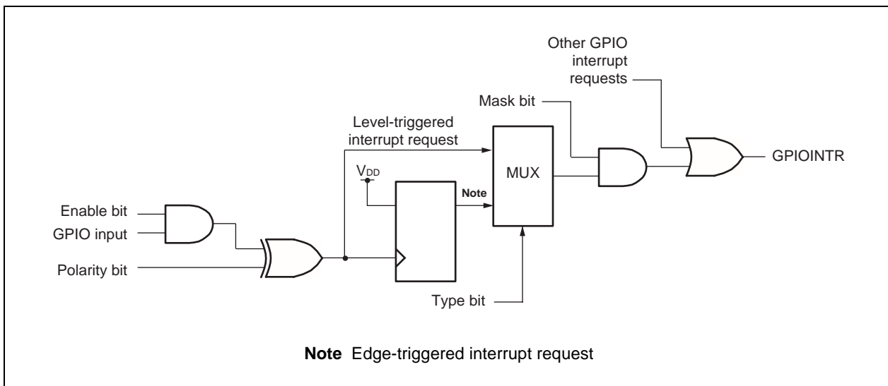
Figure 18-1. GPIO(15:0) Interrupt Request Detecting Logic
