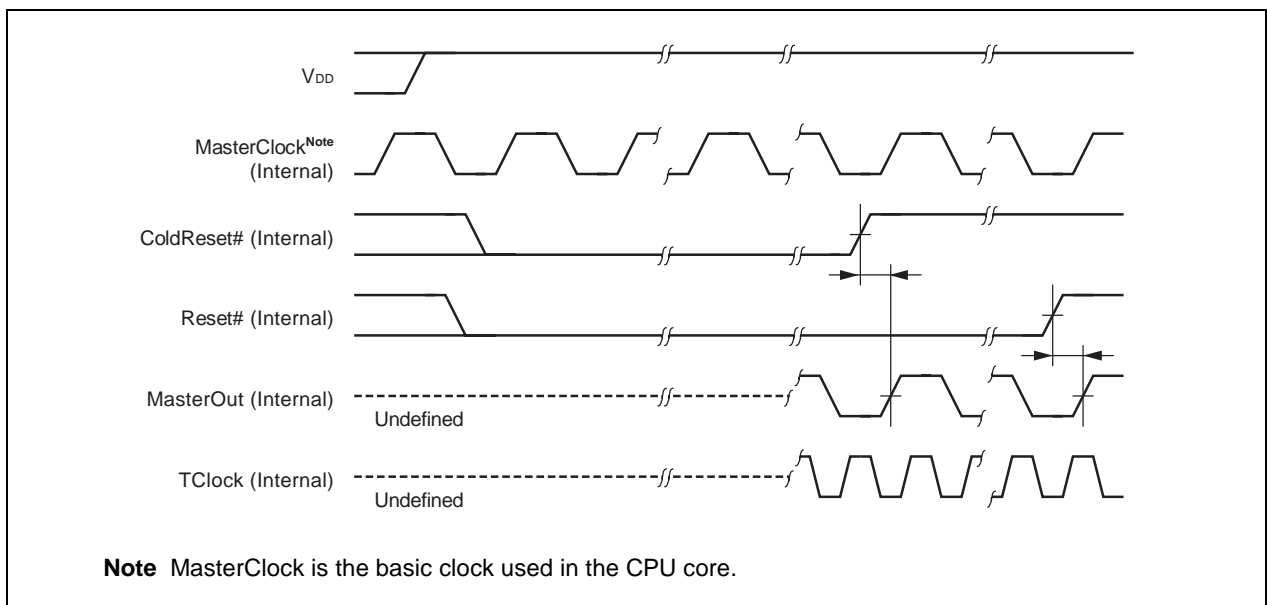
Figure 8-8. Cold Reset
