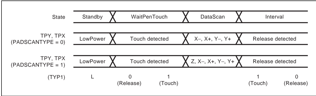
Figure 19-6. Touch/Release Detection Timing
