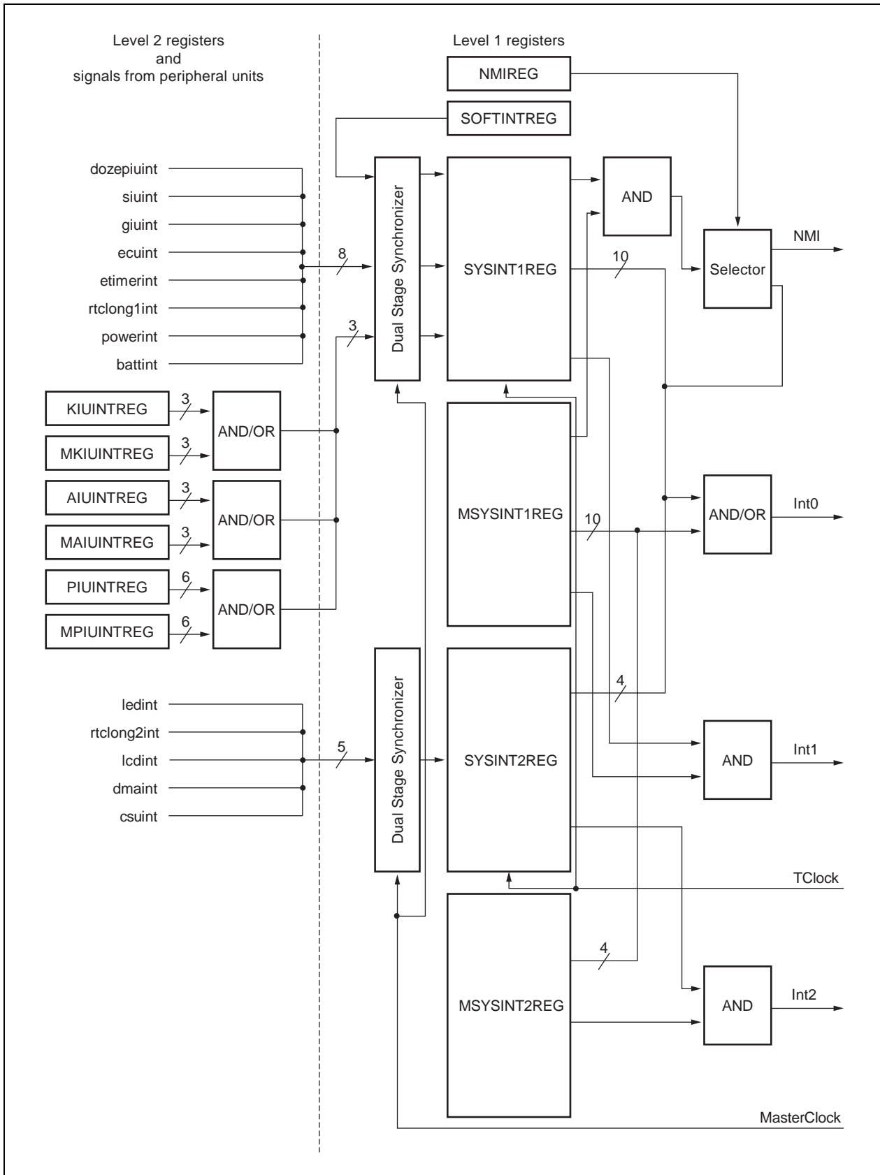
Figure 14-1. Peripheral Logic Block Assignment for Interrupt Registers
