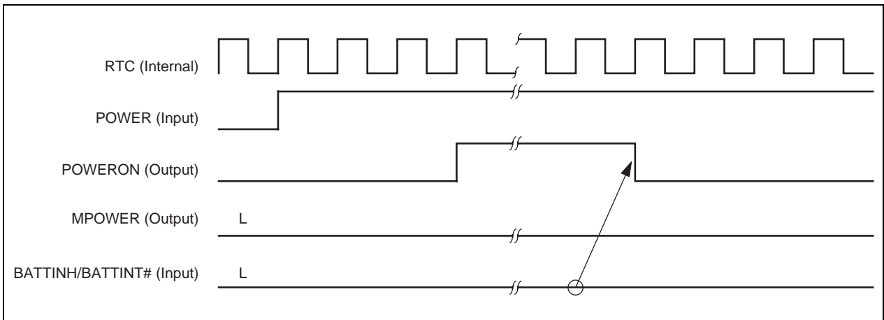
Figure 15-3. Activation via Power Switch Interrupt Request (BATTINH = L)
