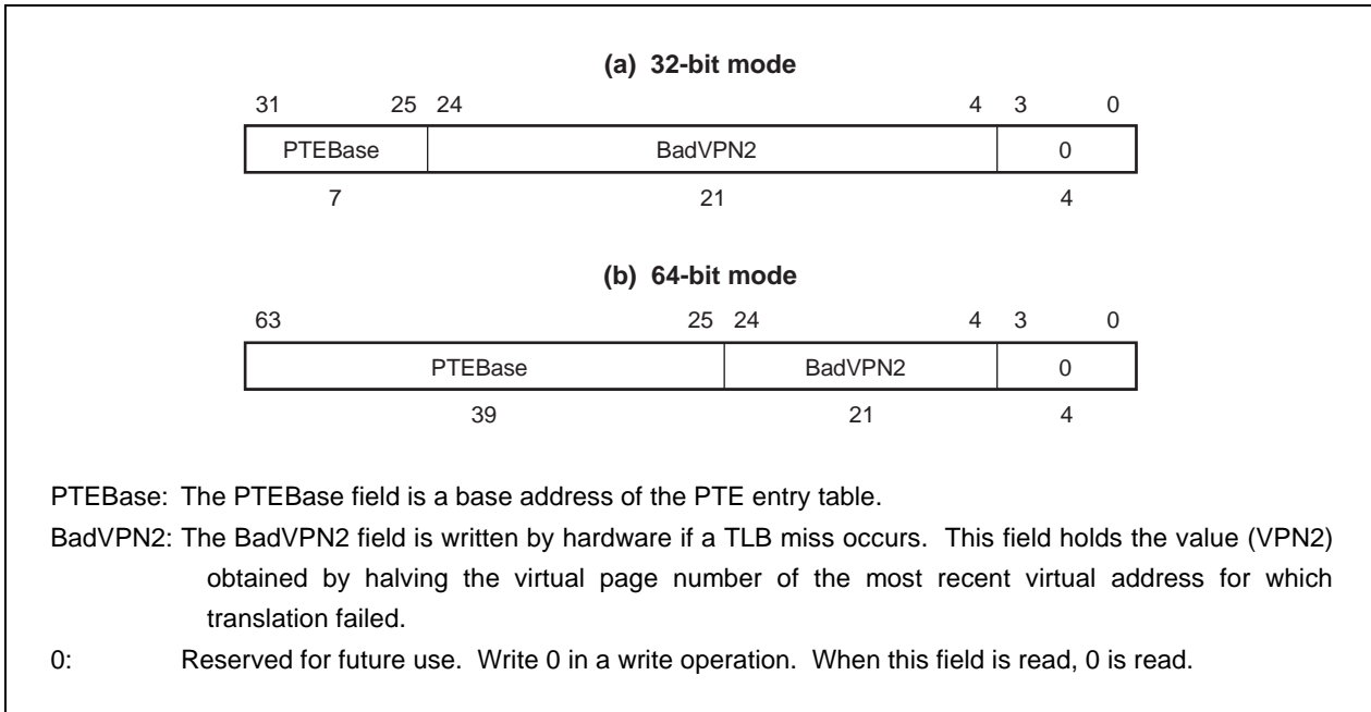
Figure 7-1. Context Register Format
