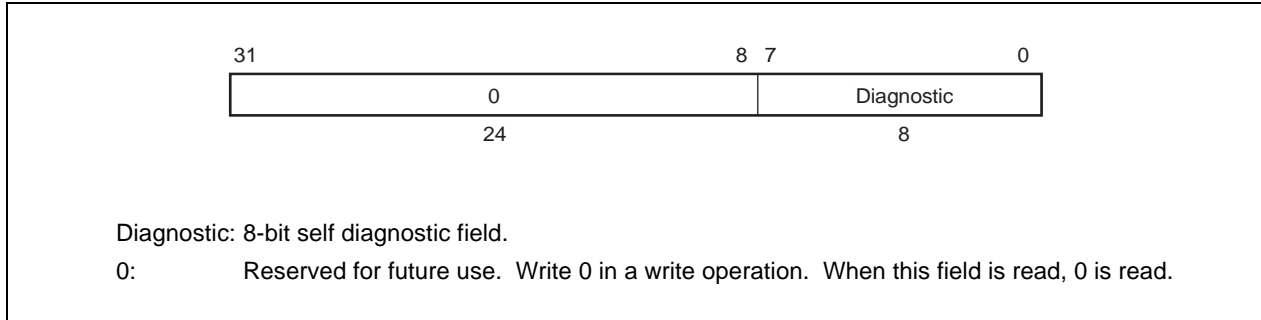
Figure 7-13. Parity Error Register Format
