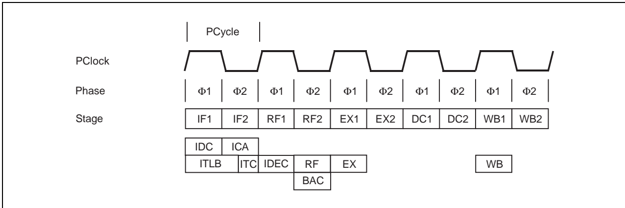
Figure 5-6. JALR Instruction Pipeline Activities
