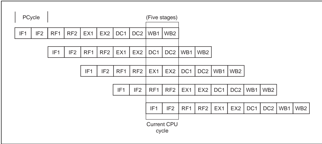
Figure 5-2. Instruction Execution in the Pipeline
