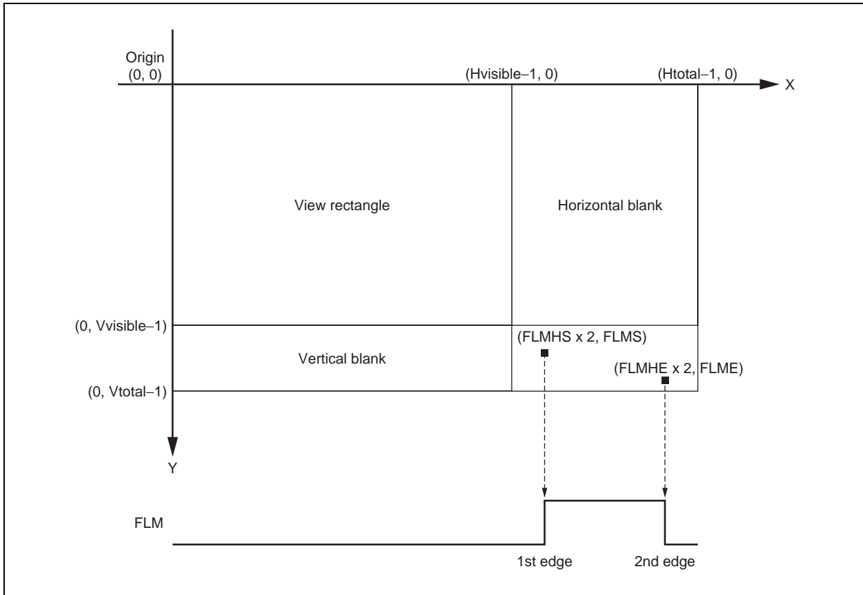
Figure 26-4. Position of Frame Edge, FLM
