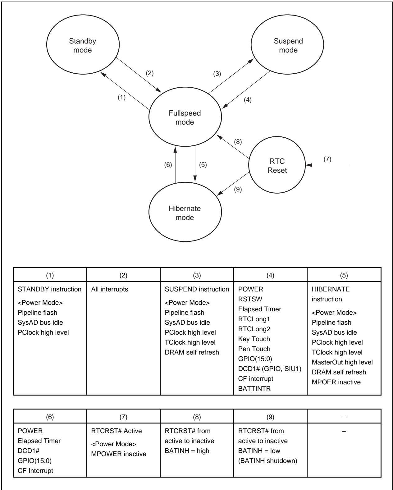
Figure 15-12. Transition of Vr4181 Operating Mode (Power Mode)
