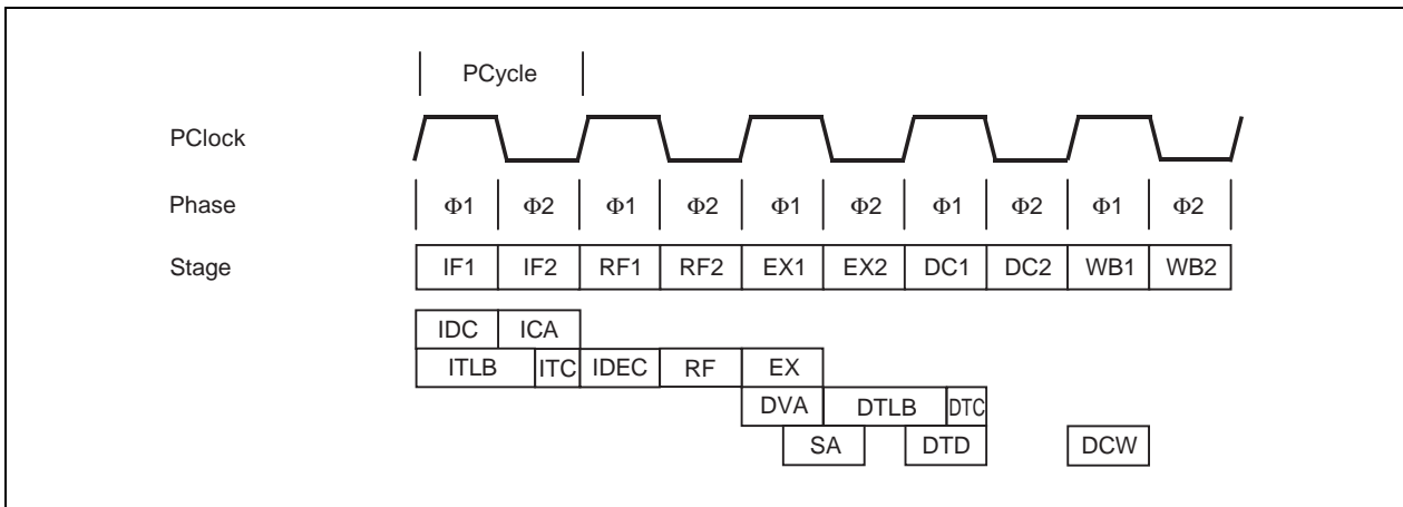
Figure 5-10. SW Instruction Pipeline Activities
