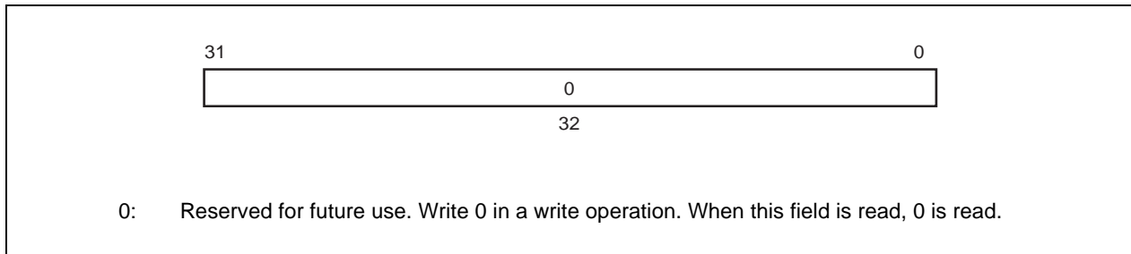
Figure 7-14. Cache Error Register Format
