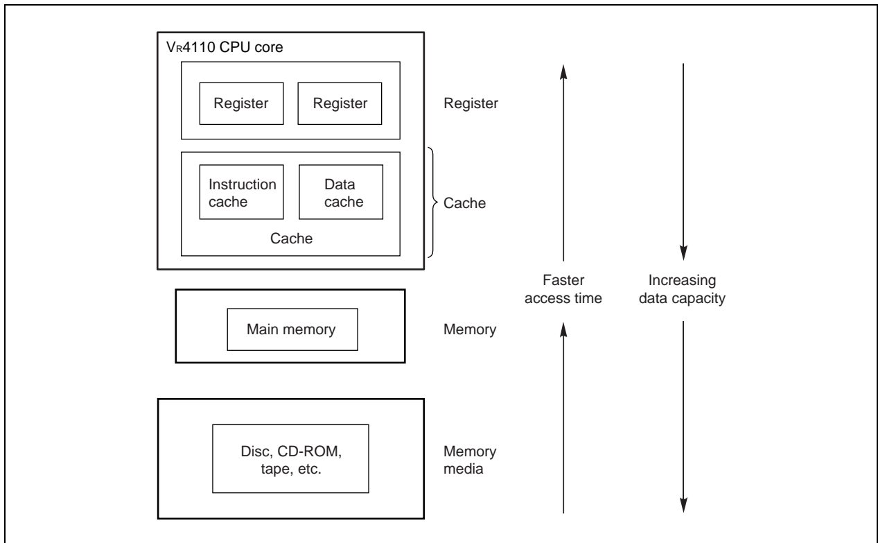
Figure 9-1. Logical Hierarchy of Memory
