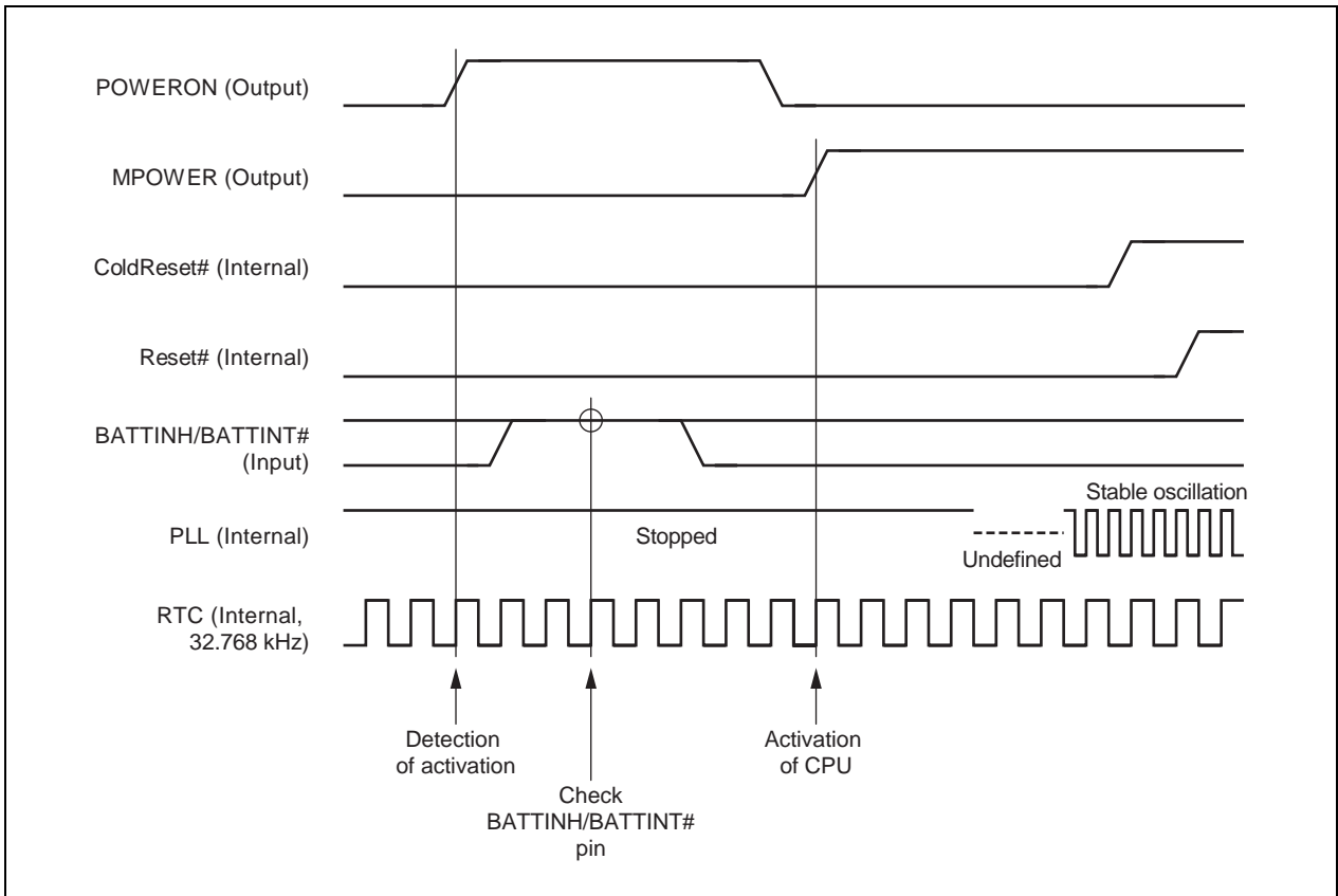
Figure 8-6. Vr4181 Activation Sequence (when activation is OK)
