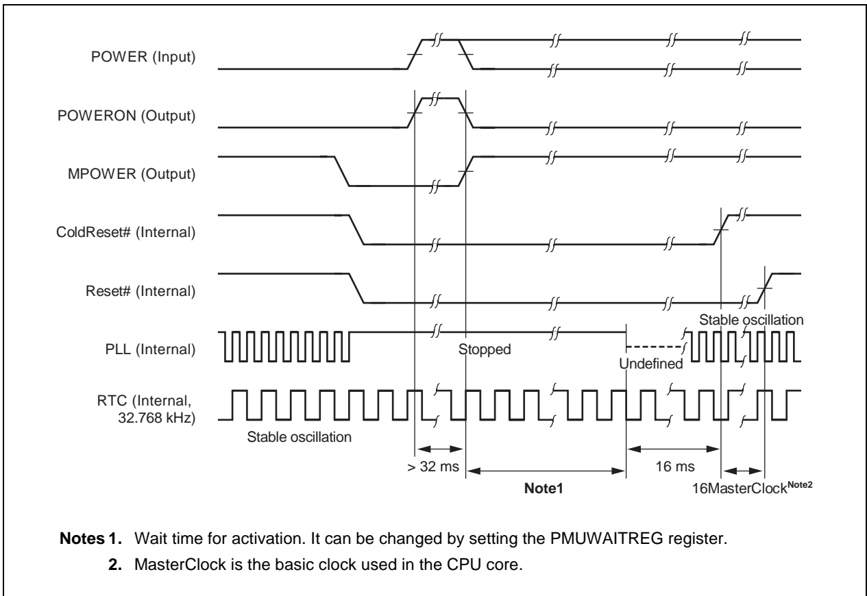
Figure 8-4. Software Shutdown
