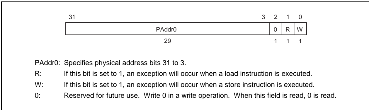
Figure 7-10. WatchLo Register Format
