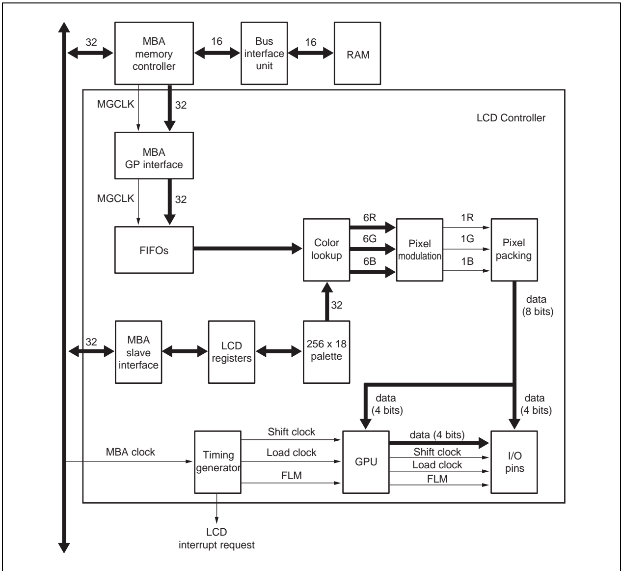
Figure 26-1. LCD Controller Block Diagram
