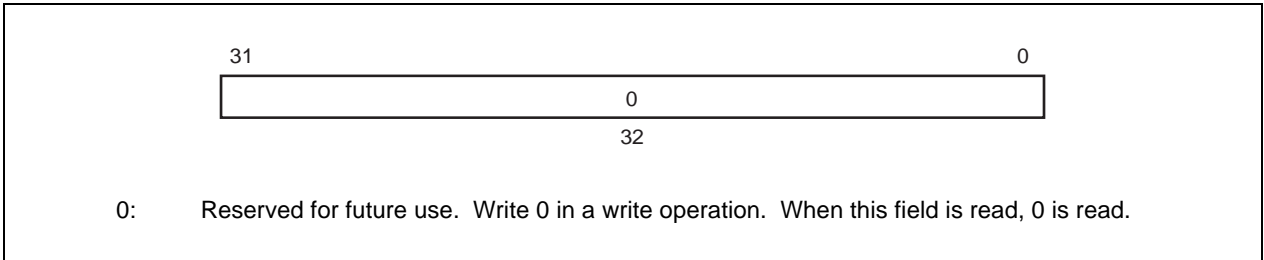
Figure 7-11. WatchHi Register Format
