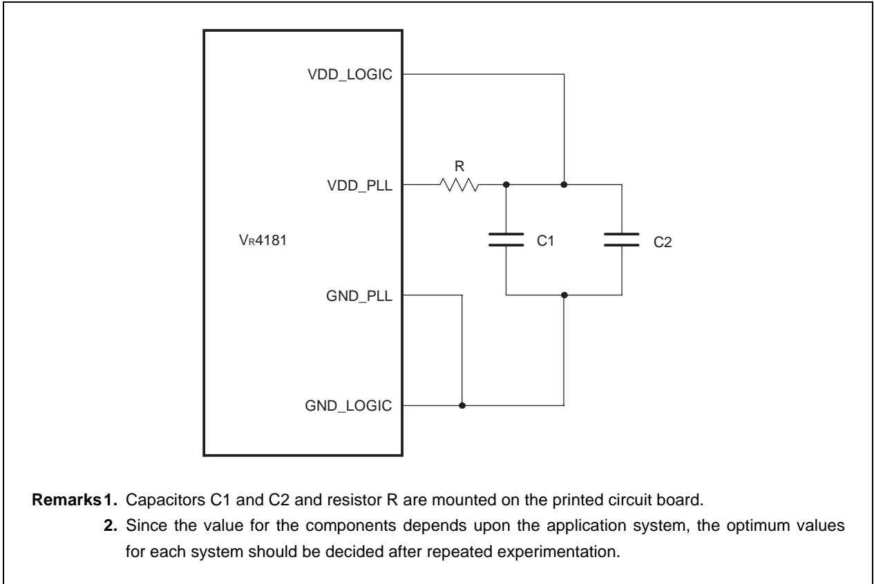
Figure 30-1. Example of Connection of PLL Passive Components
