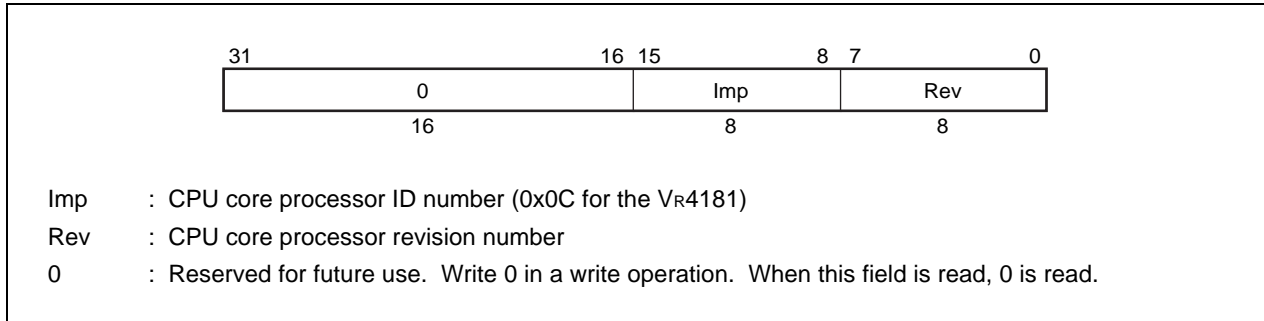
Figure 6-18. PRId Register
