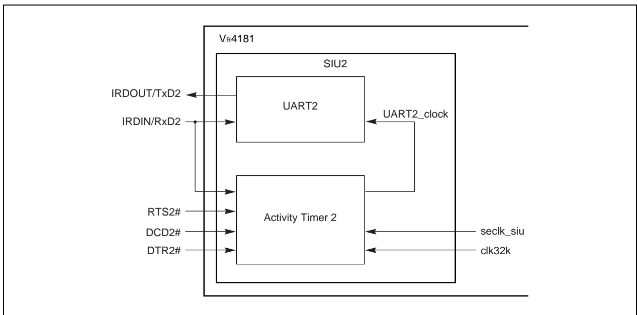
Figure 25-1. SIU2 Block Diagram
