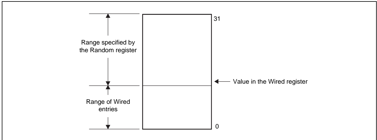
Figure 6-15. Positions Indicated by the Wired Register
